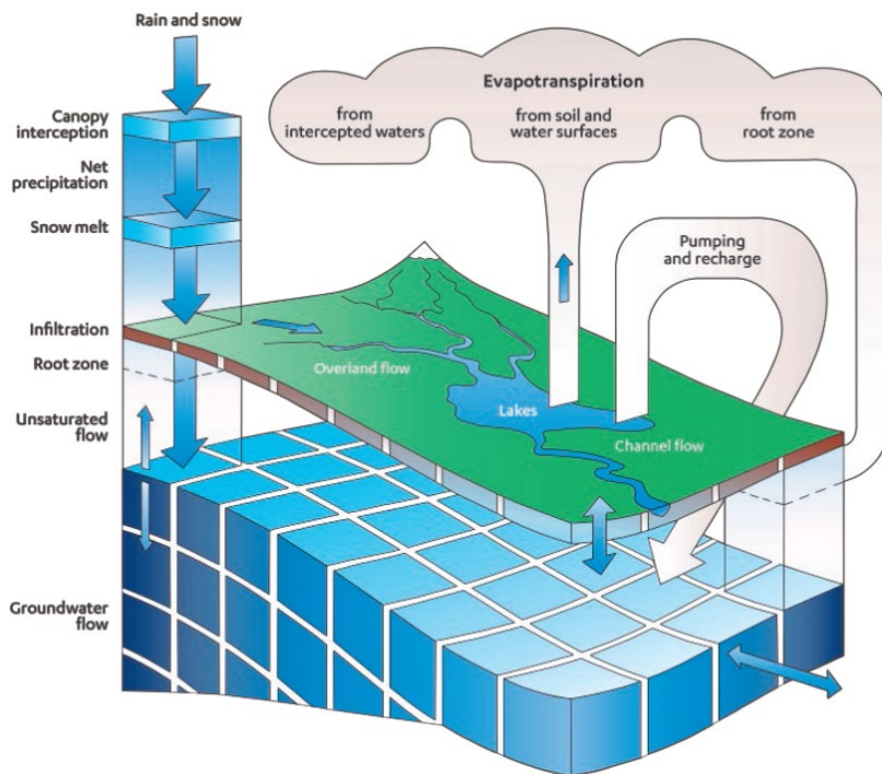
Figure 4.2 MIKE SHE model: Simulated hydrological water fluxes.
