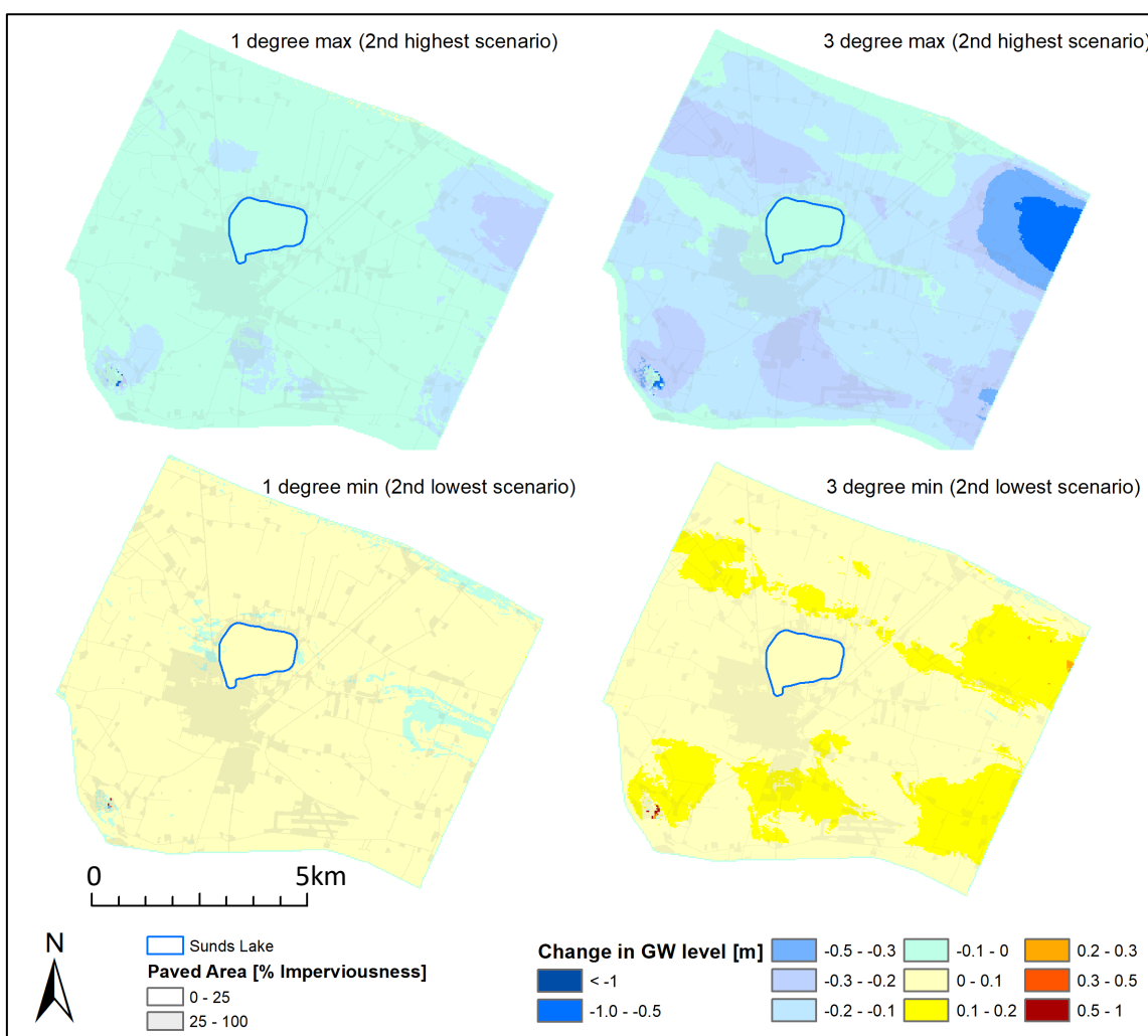
Figure 4.6 Change in groundwater levels for the four TACTIC climate change standard scenarios. The lower ones are the dry scenarios where groundwater levels mostly decrease (yellow-red colour) and the upper ones are the wet where groundwater levels increase (blue colour). Negative numbers (-) indicate an increase groundwater levels. Positive numbers indicate a decrease of the groundwater levels.
