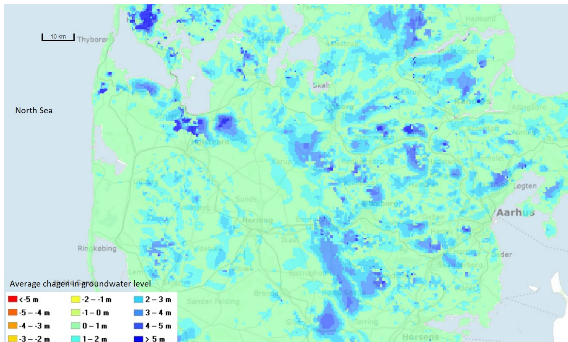
Figure 3.5 Climate change impact on groundwater. Groundwater changes between the historic period of 1961-1990 and the future period of 2021-2050. Results are shown from Central Jutland in meter of change between present and future mean groundwater table (Source: Klimatilpasning.dk 2011).
