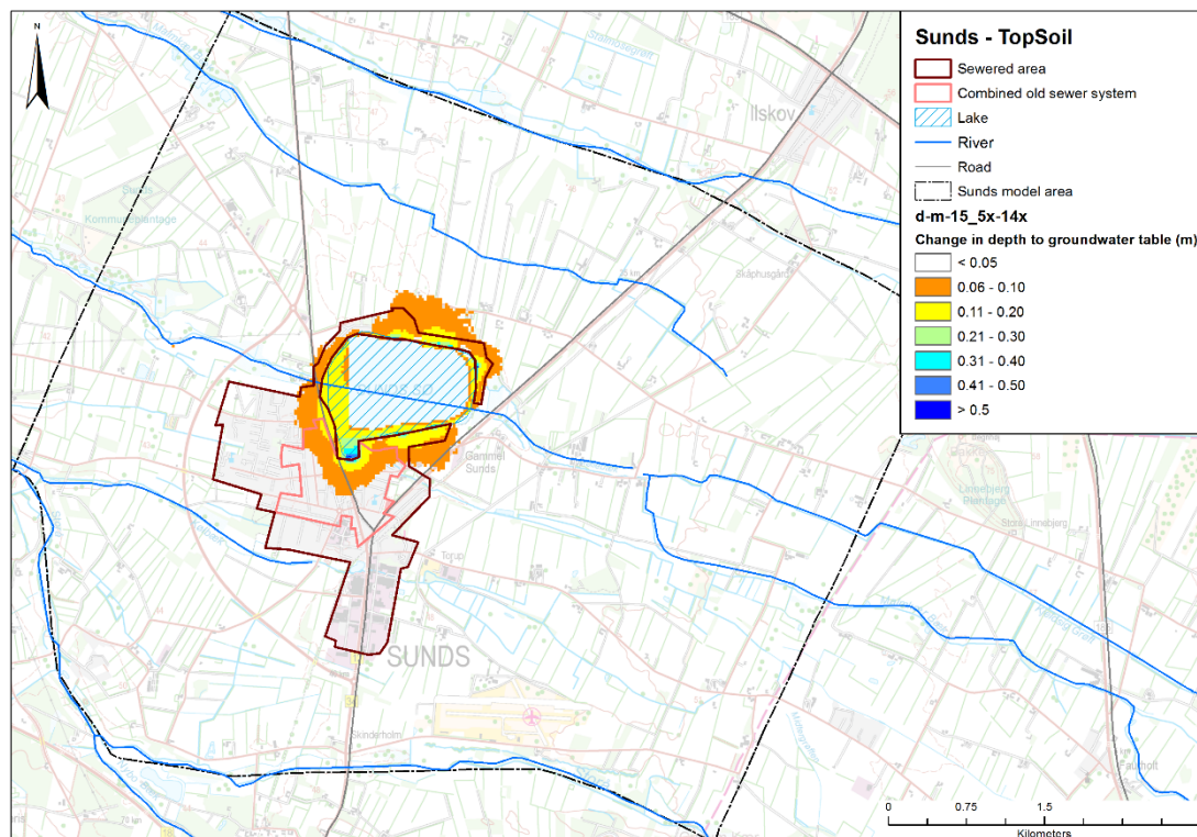
Figure 4.12 Lowering the water table in Sunds Lake to a constant elevation of 41.6 m, “the summer level”. The figure shows the situation for a median groundwater table. Rasmussen et al 2020.
