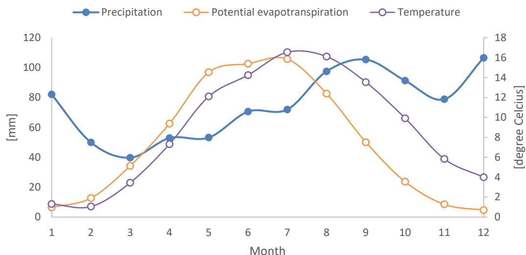
Figure 3.2 Monthly variation in precipitation, potential evapotranspiration and temperature. Average monthly values are derived from the grid-based dataset for the period of 2011-2018.
