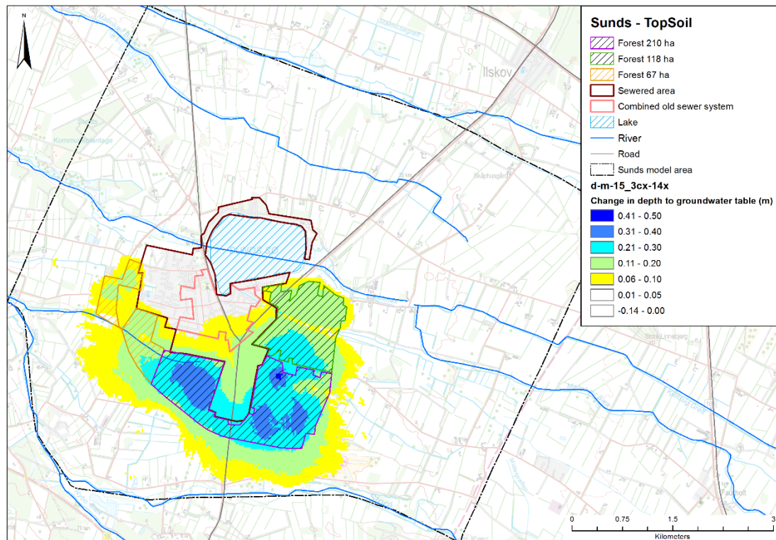
Figure 4.8 Effect on groundwater table with plantation of coniferous forest on 395 ha west, south, and east of town. Rasmussen et al 2020.
