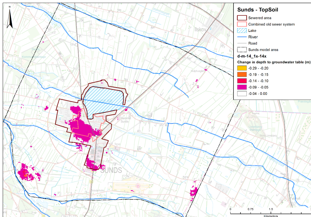
Figure 4.10 Change in depth to groundwater for the scenario with an increase of local rainwater infiltration in the whole town from 25% to 50%. Rasmussen et al 2020.
