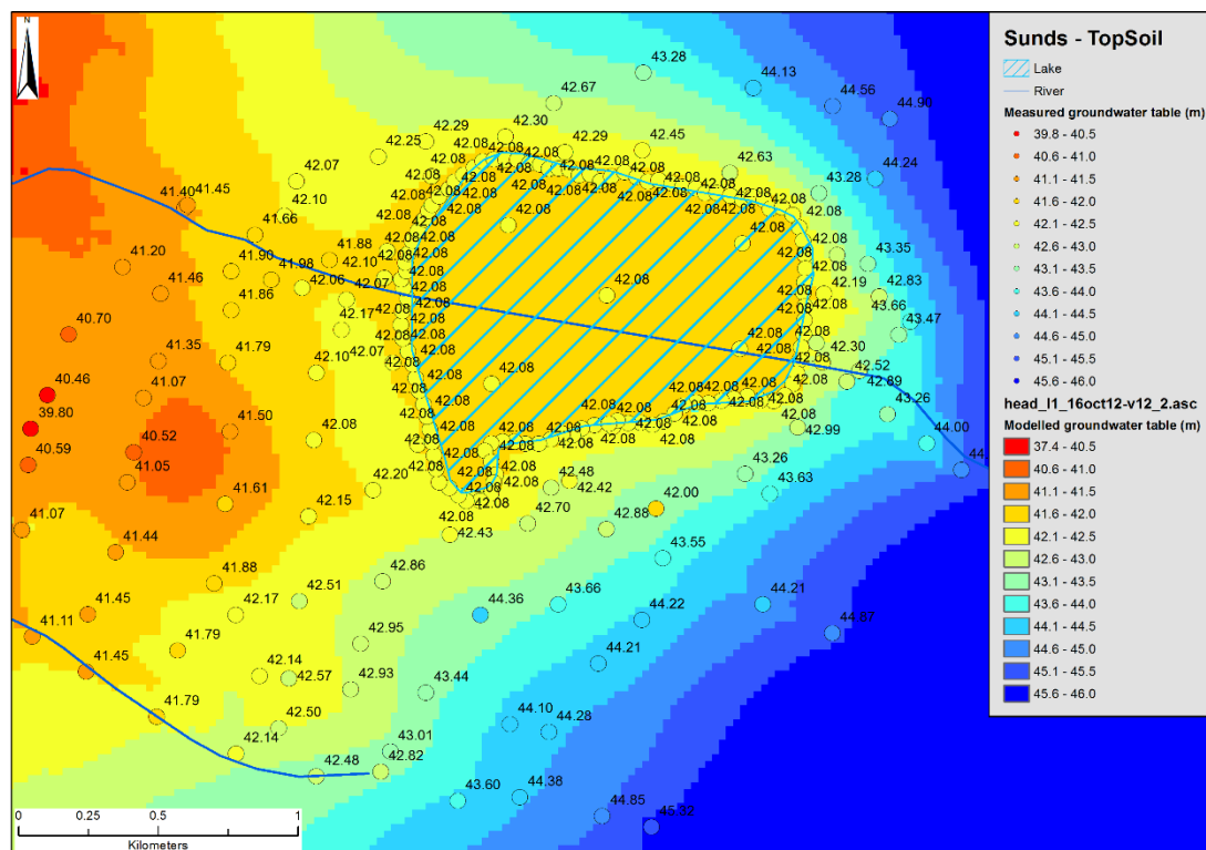
Figure 4.4 Groundwater head elevations from the calibrated hydrological model (colour contours) and the observed groundwater heads and water levels of Sunds Lake (coloured circles and numbers). Rasmussen et al. 2020.
