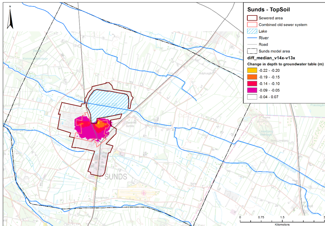
Figure 4.11 Change in depth to groundwater table after renovation of sewers in the centre of town (area inside light red lines). Rasmussen et al 2020.
