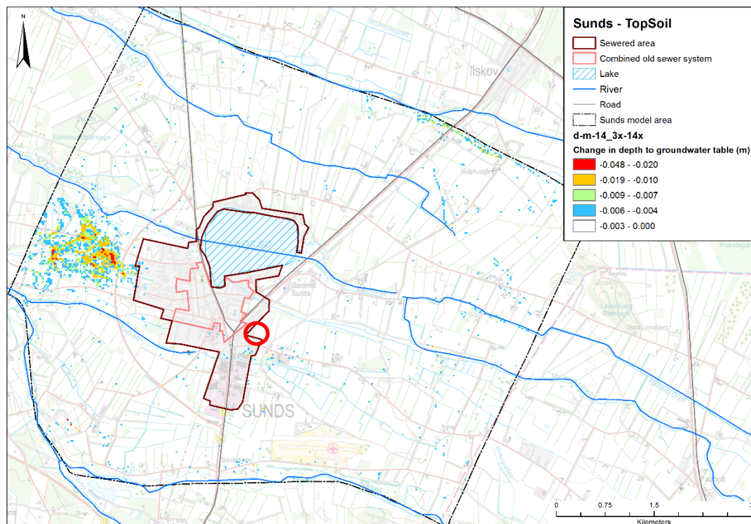
Figure 4.1 Effect on depth to groundwater table if groundwater abstraction for Sunds Waterworks stops. Minus in the numeric scale indicates a rise in groundwater table. Red circle shows the location of the waterworks wellfield. Rasmussen et al 2020.
