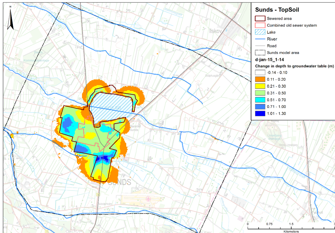
Figure 4.7 Effect on depth to groundwater table if establishing drains (3 rd pipe) in the whole town. The figure shows the situation for a January situation with high groundwater table. Rasmussen et al 2020.
