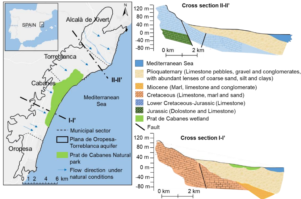
Fig. 2 Situation of the study area and hydrogeological sections
