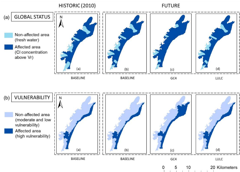
Fig. 4 Maps of affected areas in the years with the largest affected volume (a) chloride concentration and (b) vulnerability
