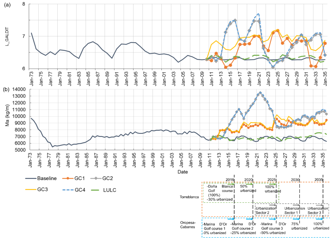
7 8 Fig. 7 Lumped indices for vulnerability and global status: (a) L_GALDIT index; (b) Ma index
