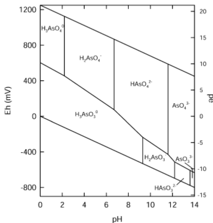
Figure 1. Eh-pH diagram for aqueous As species in the system As–O 2 –H 2 O at 25 °C and 1 bar total pressure (Smedley and Kinniburgh, 2002).
