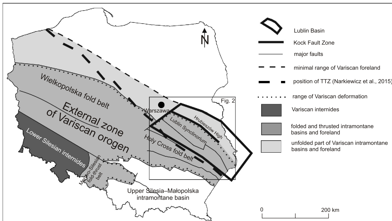
Fig. 1. Location of the Kock Fault Zone on the Variscan structure map of Poland (after Aleksandrowski and Buła, 2017, simplified)
