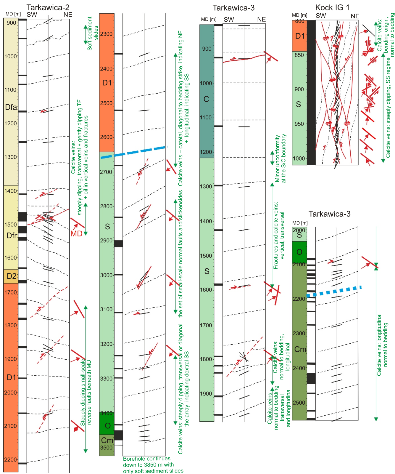
Fig. 11. Tectonic profiles of boreholes, showing results of structural study of drill core from the Tarkawica-2, Tarkawica-3 and Kock IG 1 boreholes
