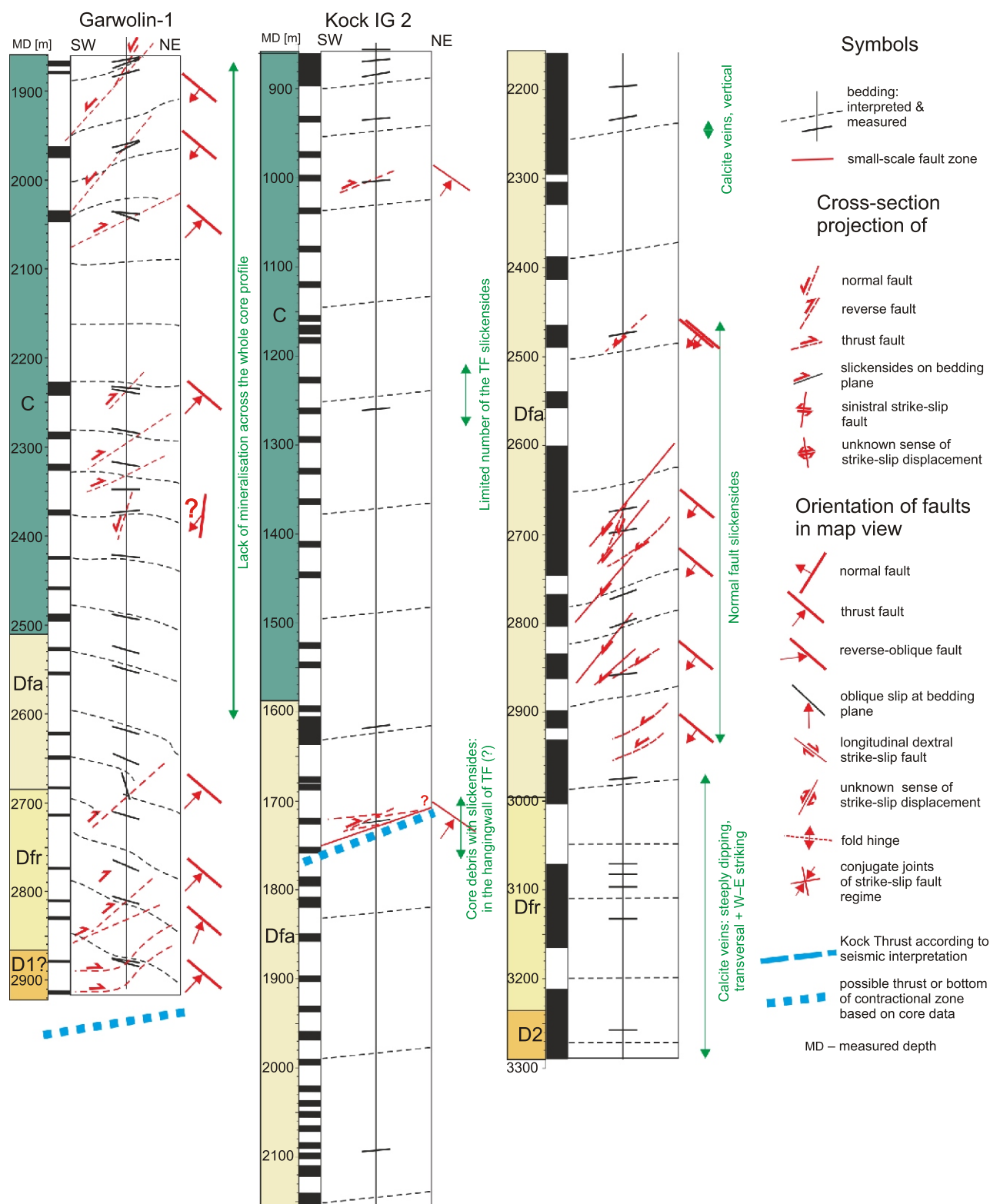
Fig. 10. Tectonic profiles of boreholes, showing results of structural study of drill core from the Kock IG 2 and Garwolin-1 boreholes
