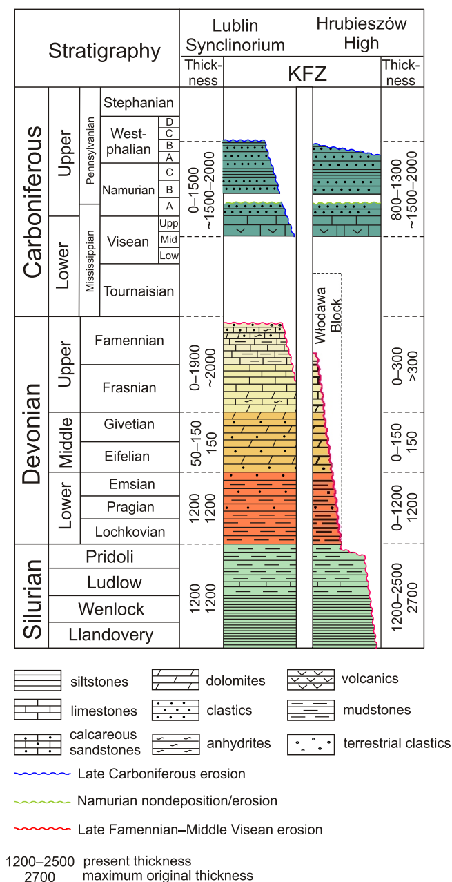
Fig. 5. Schematic lithostratigraphic profiles of the study area, showing sedimentary changes across the Kock Fault Zone
