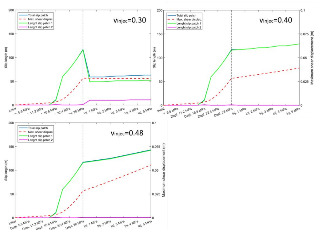
Figure 34: Evolution of maximum relative shear displacement and fault slip length during depletion and injection, for the scenarios with a Poisson's ratio of v_{inj}=0.3 , v_{inj}=0.4 and v_{inj}=0.48 during injection. Using higher Poisson's ratios during injection to model the irreversibility of the stress path can lead to the growth of the total slip length and increased relative shear displacement. The increases in slip length and maximum relative shear displacement during injection are of the same order of magnitude as during depletion.
