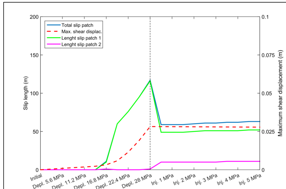
Figure C 2: Evolution of slip length and maximum relative shear displacement for the scenario of mechanism 3 with v_{injection} = 0.30 .
