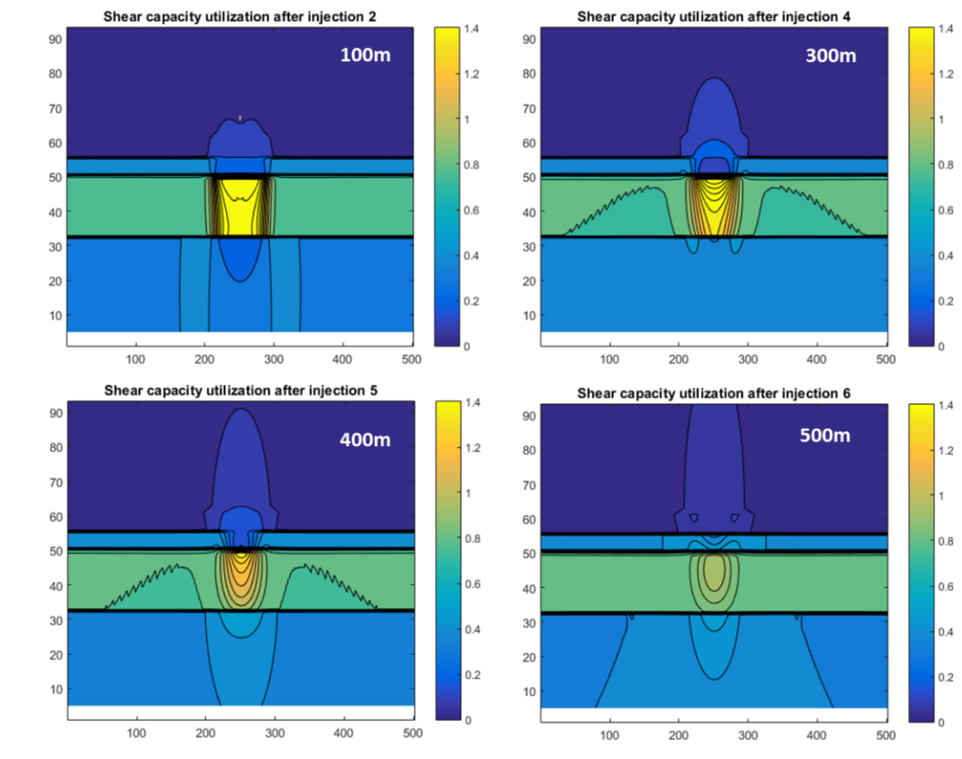
Figure D 2: Shear capacity utilization (SCU) projected onto a fault plane at distance of 100 m, 300 m, 400 m and 500 m from the injection well. Faults dip at 60^\circ away from the injection well.
