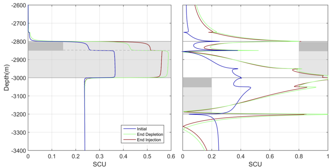
Figure 30: Shear capacity utilization SCU: Solid lines represent SCU for the scenario of 0 m offset (left) and 200 m offset (right). The light-grey blocks on the left and right indicate the position of the reservoir (Slochteren Gas and Water) in the hanging wall and footwall respectively. The dark-grey blocks indicate the position of the low-permeability Ten Boer layer.
