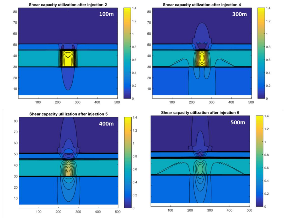
Figure D 1: Shear capacity utilization (SCU) projected onto a fault plane at distance of 100 m, 300 m, 400 m and 500 m from the injection well. Faults dip at 75^\circ away from the injection well.
