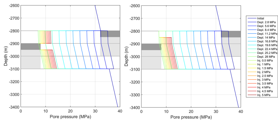
Figure 14: Evolution of pore pressures outside the fault at the start of depletion and during depletion and injection, (left) hanging wall and (right) footwall block. Light-grey blocks on the left and right indicate the position of the Slochteren Sandstone reservoir in the hanging wall and footwall respectively. Dark-grey blocks indicate the position of the Ten Boer claystone in the hanging and footwall block. The change in slope is caused by the difference in density between water and gas. Geometry and pore pressures for the base case scenario of 100 m fault offset.
