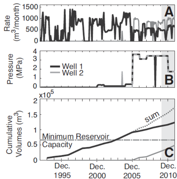
Figure 10. Injection data for the Wilzetta Oil Field, Prague, Oklahoma. A) Monthly volumes of waste water injected into two wells close to the nucleation of the first M_w=5.0 seismic event. B) Wellhead pressures for active pumping periods. C) Cumulative volumes injected. The dashed line shows the minimum reservoir capacity, which equals the estimated total oil volume produced. Gray shading represents the occurrence of the 2010-2011 earthquakes. Source: Keranen et al. (2013).
