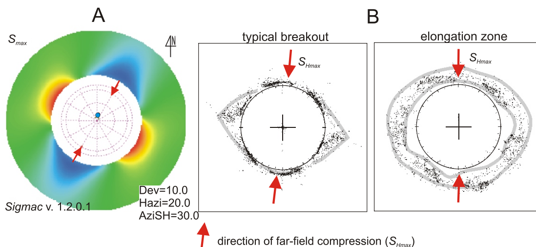
Fig. 2. A — stress disturbance around borehole in the plane perpendicular to the well axis obtained with SIGMAC computer program; the maximum effective principal stress ( S_{max} ) values are shown (high in red, low in blue, far-field stress value in green); B — approximate borehole cross-sections represented by caliper pad projections in the SPIDER program processing. Typical breakouts, being the best indicator of the S_{Hmax} direction, develop when only part of the borehole fails. Elongation zones, also regarded as tectonic stress indicators, develop when the whole circumference of the borehole fails. Usually in this case the azimuth of S_{Hmax} is determined with less precision
