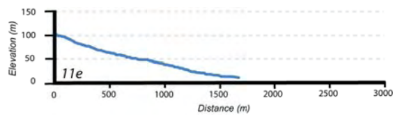
Longitudinal drainage profile for basin 11e (Vertical exaggeration 5x)
