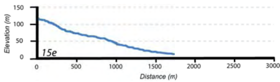
Longitudinal drainage profile for basin 15e (Vertical exaggeration 5x)
