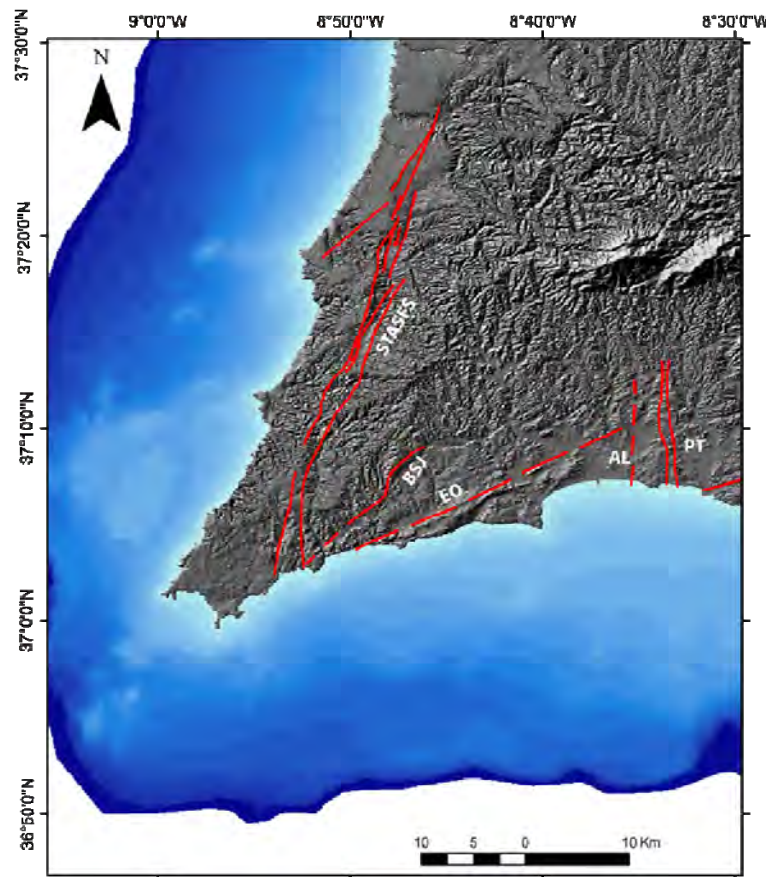
Figure 1.2 - São Teotónio-Aljezur-Sinceira fault system (STASFS) and other main Plio-Pleistocene faults like Barão de São João (BSJ), Espiche-Odiáxere (EO), Alentejo-Placencia (AL) and Portimão (PT) overlapping an ASTER shaded relief DTM. Bathymetric information until 200 m depth also included (adapted from Dias, 2001).
