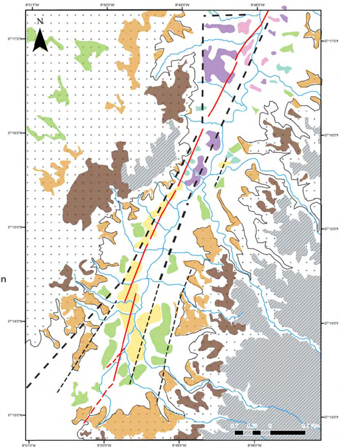
I.I Morphotectonic map for Aljezur- Alfambras basin, south sector
