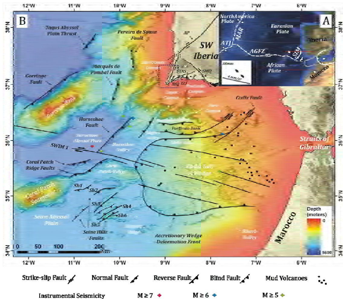
Figure 1.7 – Main active structures and morphological features in the Southwest Iberia region (according to Rosas et al. 2012, and Martínez-Loriente et al. 2013, for the offshore, and Dias, 2001, for the onshore) and their localization regarding the Eurasia – Nubia plate boundary. (A): Schematic Eurasia- Africa Plate boundary for the region and localization of figure 1 MAR - Mid - Atlantic Ridge; ATJ- Azores Triple Junction; AGFZ – Azores Gloria fault zone; SIM – Southwest Iberian Margin (adapted from Duarte et al. 2013); (B) Offshore structures identified in the map; onshore structures : AP – Alentejo- Placencia Fault; STAS – São Teotónio-Aljezur-Sinceira Fault System; BSJ – Barão de São João Fault; EO – Espiche –Odiáxere Fault; P – Portimão Fault; SMQ – São Marcos-Quarteira Fault. The area studied in this work is delimited by the dashed line (adapted from Rosas et al. , 2012, in Figueiredo et al. 2013).
