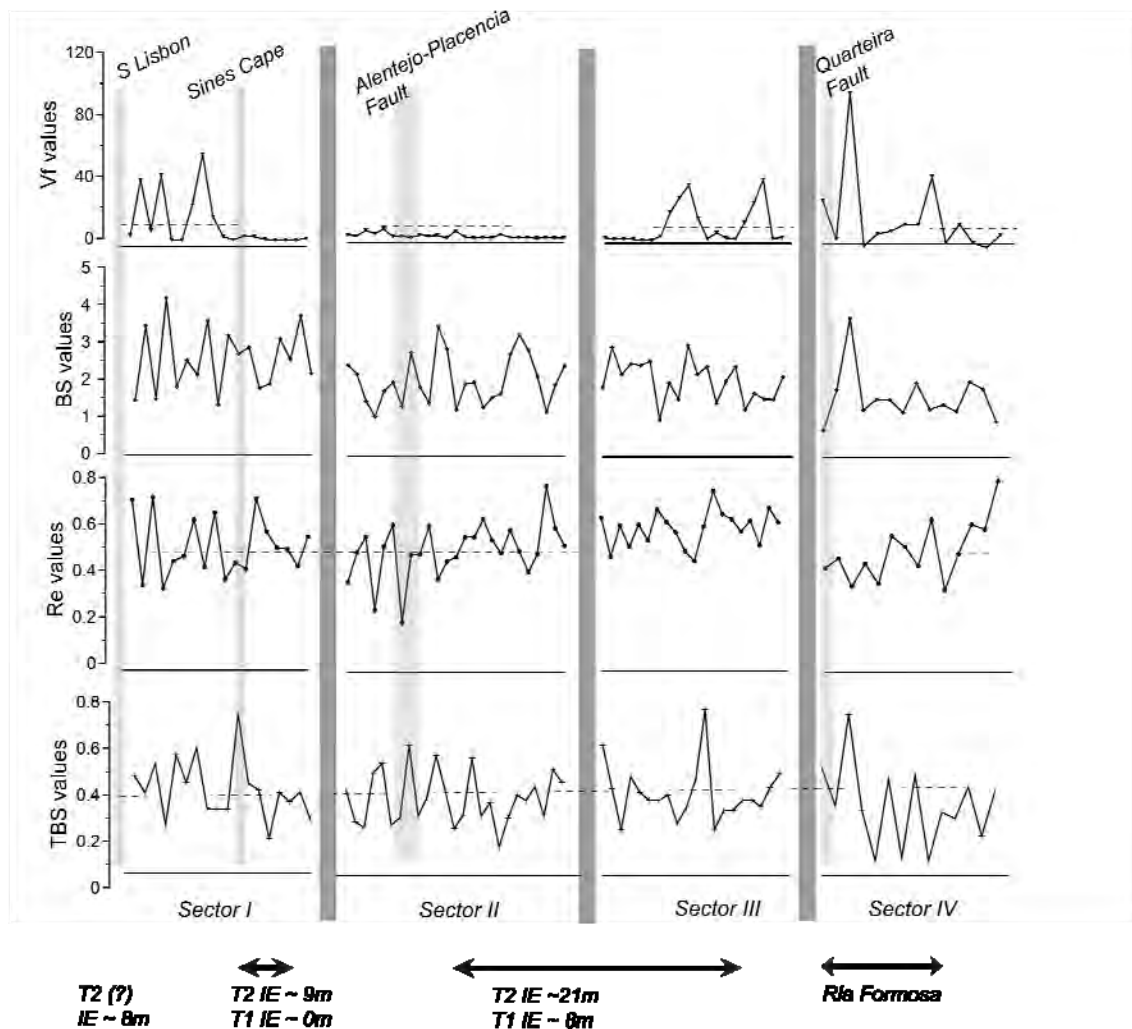
Figure 4.4 – Plots of the results for all the sectors for basin shape indexes and Valley-floor width. Further information relative a geographical reference, main structures and marine terraces inner edges present along the coastline is also included.
