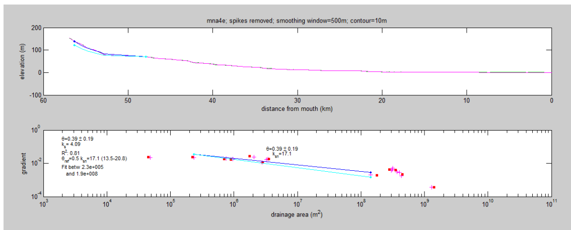
Longitudinal profile, area- length relationship, gradient-area relationship and values of concavity and Ksn obtained for channel 4e.
