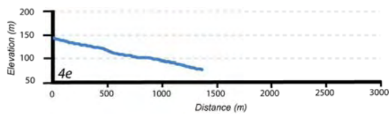
Longitudinal drainage profile for basin 4e (Vertical exaggeration 5x)
