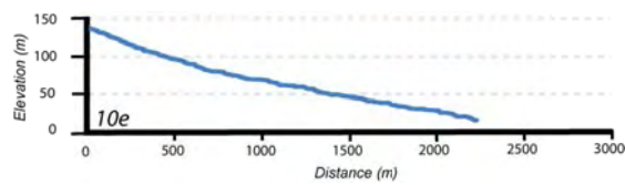
Longitudinal drainage profile for basin 10e (Vertical exaggeration 5x)
