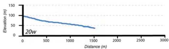
Longitudinal drainage profile for basin 20w (Vertical exaggeration 5x)
