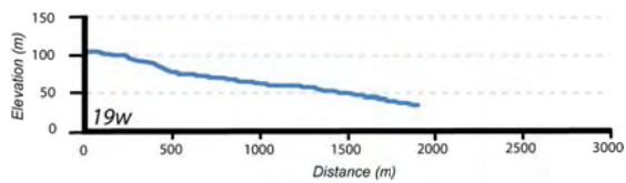
Longitudinal drainage profile for basin 19w (Vertical exaggeration 5x)
