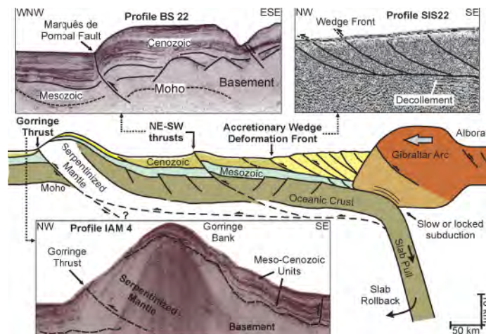
Figure 1.5 – Crustal sections interpretations from the Southwest Iberia Margin and Gibraltar Arc according to Duarte et al. , 2013: westward Gibraltar Arc main active structures along the Gulf of Cadiz and Southwest Iberia margin are depicted (adapted from Duarte et al. 2013)
