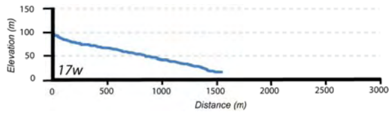
Longitudinal drainage profile for basin 17w (Vertical exaggeration 5x)
