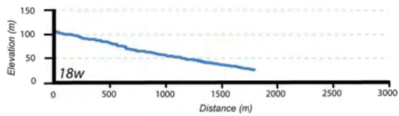
Longitudinal drainage profile for basin 18w (Vertical exaggeration 5x)
