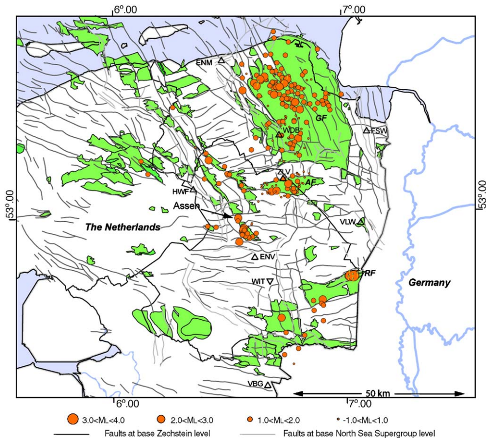
Fig. 4. A schematic figure of the hydrocarbon (gas) exploitation fields (green), the major fault structures (source: NITG), the seismometer station WIT (inverted triangle), borehole seismometers (triangles) and the seismicity (solid orange circles) in the north-eastern part of The Netherlands (inset of Fig. 1). Some of the gas fields discussed in this report are indicated: RF — Roswinkel Field; GF — Groningen Field, EF — Eleveld Field, AF — Annerveen Field. After Dost and Haak (2006).
