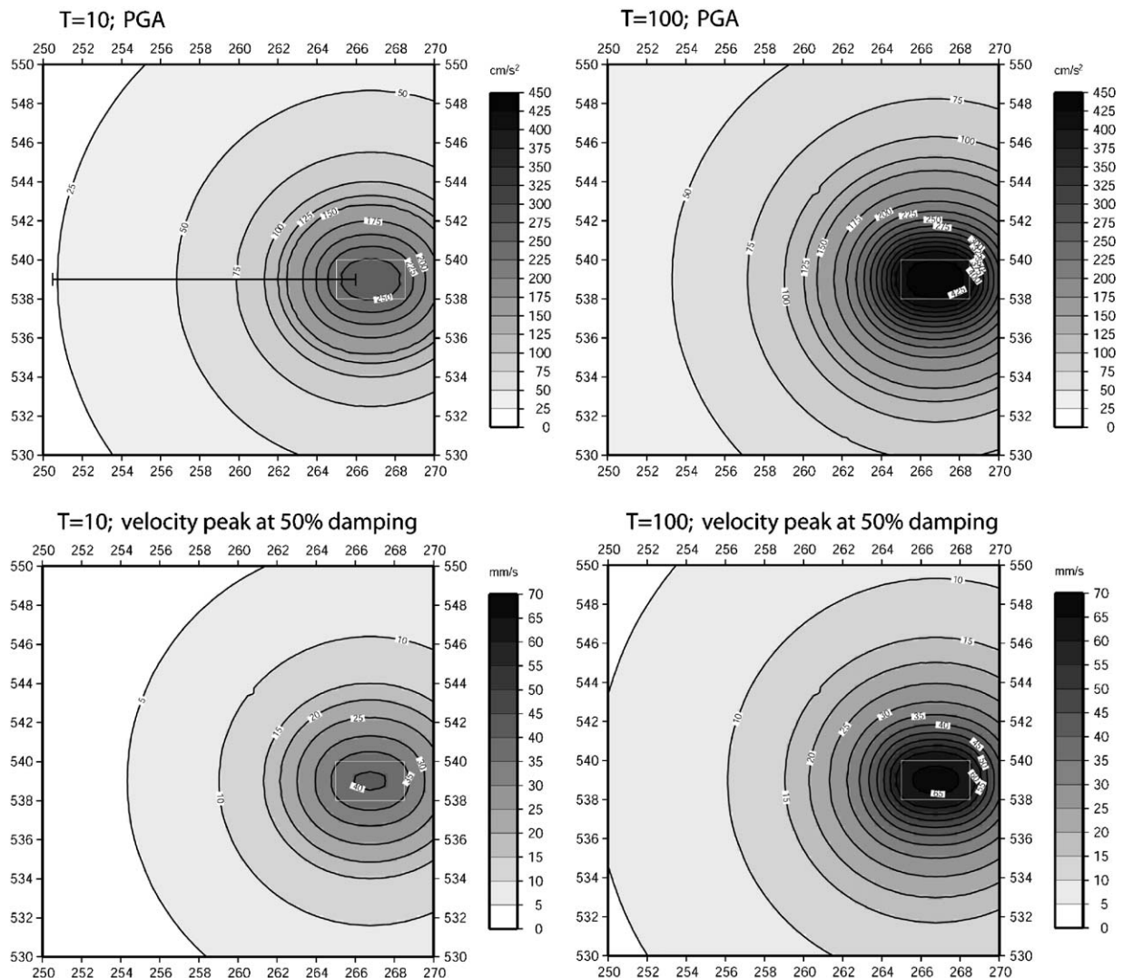
Fig. 8. Estimated hazard at and around the Roswinkle field. The hazard has been estimated for two return periods, i.e. T=10 years (left) and T=100 years (right). The hazard indicates a 10% probability that the peak values as indicated can be exceeded within 1 year ( T=10 ) and within 10 years ( T=100 ) respectively. Alternatively, the figures indicate an annual probability of 10% ( T=10 ) and 1% ( T=100 ) that the indicated peak values will be exceeded. In the following figures the hazard is only shown as a section indicated, for example, in this upper left figure. The x- and y-axis indicate distance in kilometers.
