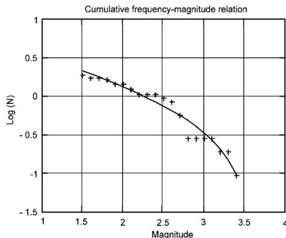
Fig. 5. Annual cumulative frequency-magnitude relation for all events associated with the Roswinkel gas field during the period 1992–November 2003 and the best fit seismicity model for all available data.
