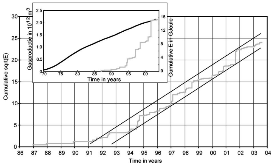
Fig. 2. Cumulative of the square root of the seismic energy (E) in Gjoule (light grey curve) of all earthquakes with M_L \geq 1.5 as a function of time. The black straight lines indicate the upper and lower energy boundaries, providing an estimate of M_{\max} = 3.8 assuming that the energy release is and remains stationary. The inlay figure compares the cumulative seismic energy release (light grey curve) with cumulative gas production on land (black curve). Gas production numbers are kindly supplied by the NITG.
