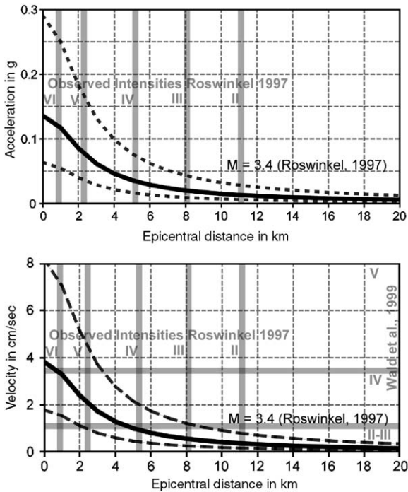
Fig. 6. Ground motion model (PGA and PGV) of Dost et al. (2004) and averaged intensity observations for the M=3.4 Roswinkel earthquake of 19 February 1997 (Dost and Haak, 1997). Also shown are the intensity values as related to the PGV by Wald et al. (1999).
