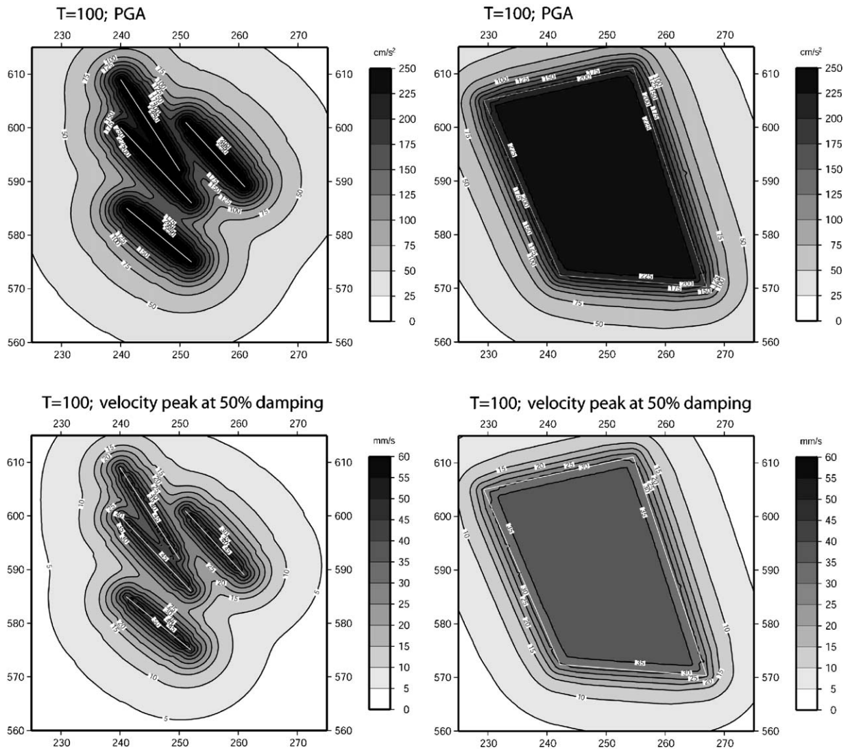
Fig. 11. Two source models used in a seismic hazard analysis for a schematic Groningen field and T=100 . To the right the seismicity is assumed to be uniformly distributed over the whole exploitation field. To the left the seismicity is assumed to be distributed over four main faults (here modeled as straight lines). Observed seismicity suggests some linear correlations that may be related to fault zones. This comparison gives an indication of the uncertainty due to the source modeling. In some areas the hazard increases in PGA from around 225 to 300–350 \text{cm/s}^2 . In other areas the hazard decreases in PGA from around 225 to about 100–125 \text{cm/s}^2 and even lower. The x - and y -axis indicate distance in kilometers.
