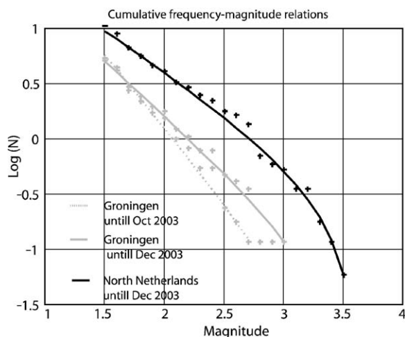
Fig. 3. Cumulative annual frequency-magnitude relation obtained for all induced seismicity in the north of The Netherlands for the period 1986–2003 (black curve) and observations (black crosses). Also is shown the same frequency-magnitude relation for all earthquakes in the Groningen field. However, for this selection we have shown the relation excluding (grey broken curve) and including (grey curve) three events 2.7 < M < 3.0 that occurred October–November 2003. This shows that the slope ( b -value) of the frequency-magnitude relation for a subset of 179 events has a tendency to approach the b -value of the frequency-magnitude relation for all earthquakes (340 events).
