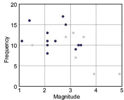
Fig. 7. Frequency at which the peak of the velocity response spectra occurs as a function of earthquake magnitude ( M_L ). The peak frequencies are measured at the horizontal components of acceleration recordings of 19 events in the Netherlands; 12 shallow induced events (black) in the northern part of The Netherlands and 7 natural seismic events (grey) in the southern part of The Netherlands. All sites are characterized as stiff soil.
