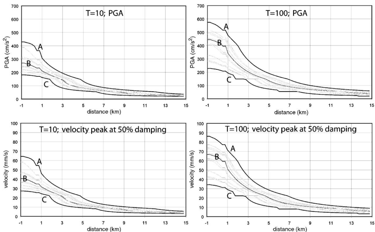
Fig. 10. Sensitivity analysis for the seismic hazard in the vicinity of the Roswinkel field for different model and parameter values. Left figures: hazard estimates for T=10 . Right figures: hazard estimates for T=100 . From top to bottom: the PGA and the peak spectral velocities 50% damping. Two extreme models (A and C) and one average model (B) are indicated in black. Other models are indicated in grey. Hazard model A (upper curve): seismicity model 1, i.e. N(M \geq 1.5)=8 , b=0.8 , M_{\max}=3.9 and \sigma=0.4 . Hazard model B (middle curve): seismicity model 2, i.e. N(M \geq 1.5)=2 , b=0.5 , M_{\max}=3.5 and \sigma=0.4 . Hazard model C (lower curve): seismicity model 2, i.e. N(M \geq 1.5)=2 , b=0.5 , M_{\max}=3.5 and \sigma=0.2 .
