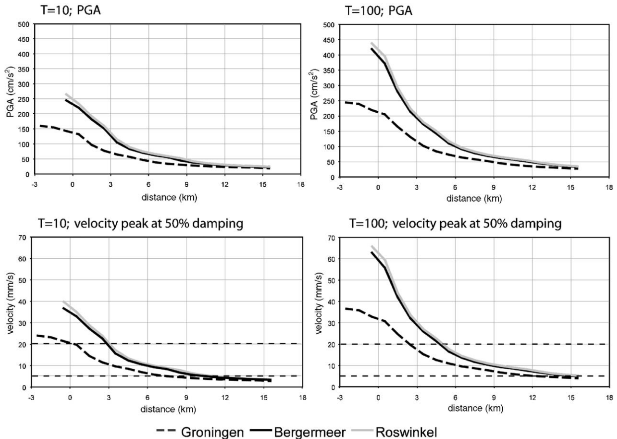
Fig. 9. Seismic hazard as a function of distance from the surface projection of the exploitation field. Three examples are shown: the Groningen, the Bergermeer and the Roswinkel field. The top two figures show the PGA for two return periods, T=10 and T=100 years. The bottom two figures show the same for the V_{\max} at 50% damping. These hazard-distance functions have been used in the pragmatic approach to obtain seismic risk estimates.
