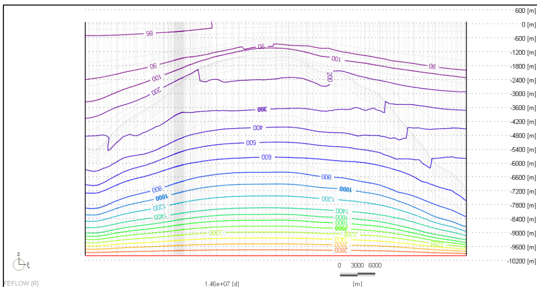
Figure 88: Modelled water level distribution (40 thousand years of run, no production) on vertical section [m.a.s.l.]
