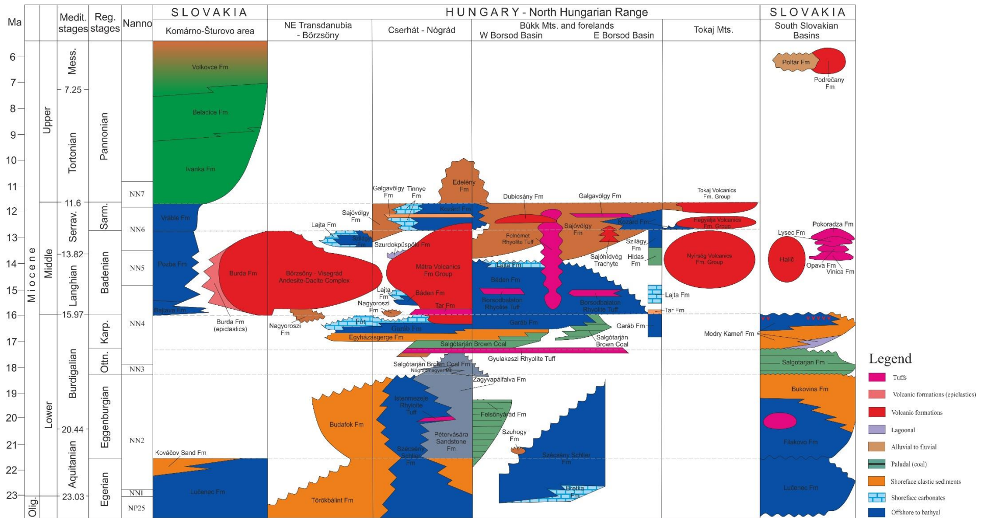
Figure 10: Harmonized stratigraphic chart between Eastern Slovakia and Hungary
