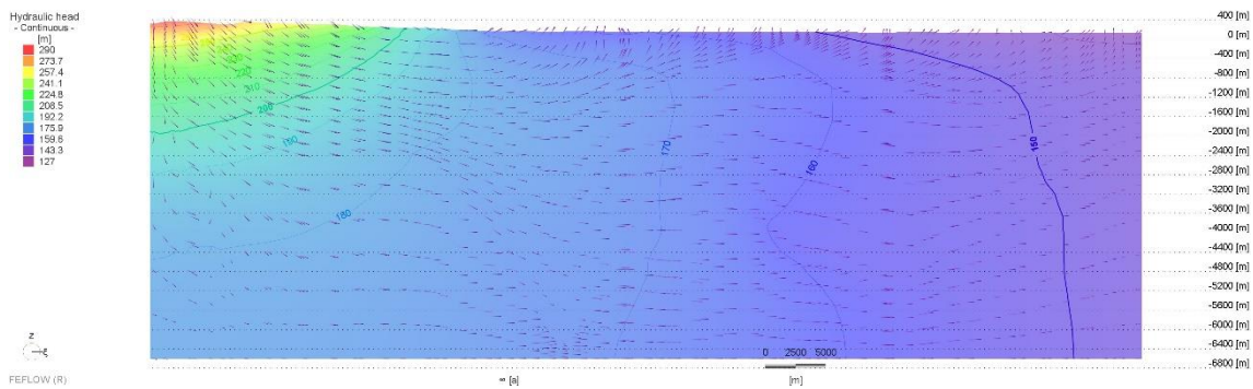
Figure 51: Hydraulic head distribution and flow direction in best fitted Scenario 4 show different heads than in Scenario 2. In Sc. 4, the flow in basement in the central part of the model is more horizontal – it represents the intermittent point of regional flow lines. The same is that recharge is in Goričko Hills area and outflow in flatlands on the southern parts. Heads are the same (very little vertical gradient) in the Ljutomer fault zone.
