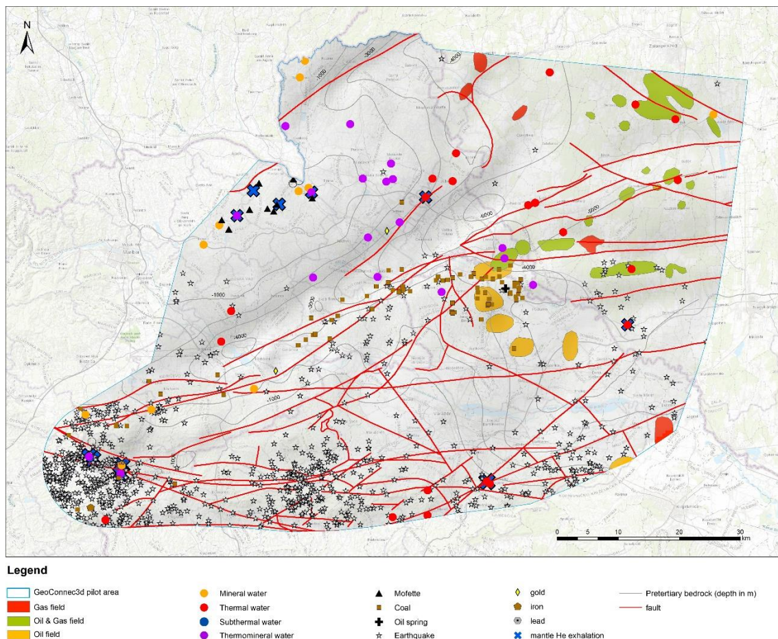
Figure 16: Presentation of all known geomanifestations in the Mura-Zala sub-basin area with newly delineated structural features (faults) within the GeoConnect3d project.
