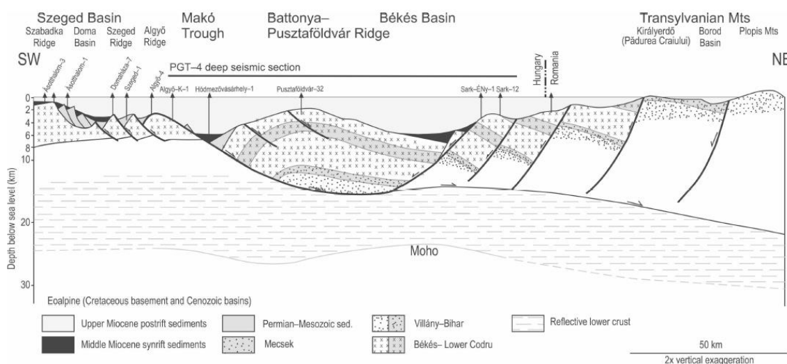
Figure 66: Regional geological profile in the south-eastern part of the Pannonian Basin (adapted from Tari et al. 1999)
