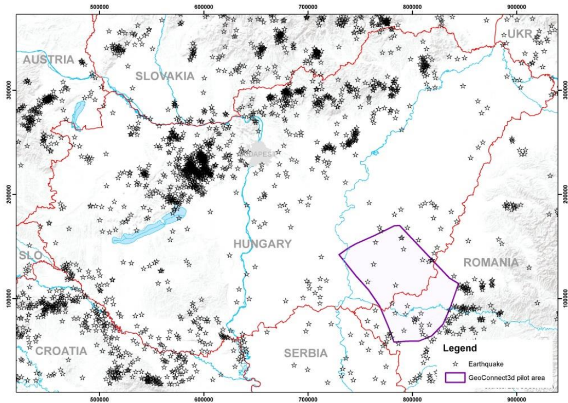
Figure 79: Seismic points (Earthquakes) of the Pannonian basin
