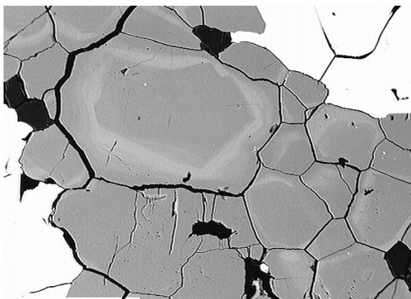
Figure 38. Back-scattered electron (BSE) image of an aggregate of fluorapatite (in different shades of grey) in magnetite-apatite ore from the Export field, Grängesberg (white areas are magnetite). The lighter zones, particularly in the fluorapatite in the centre, have increased REE content; it is suggested that the texture of this variable zoning is due to a similarly variable extent of fluid-mediated remobilisation of REEs at a late-magmatic to regional metamorphic stage. The white scale bar at lower left equals 200 micrometres. Photo: Erik Jonsson.
