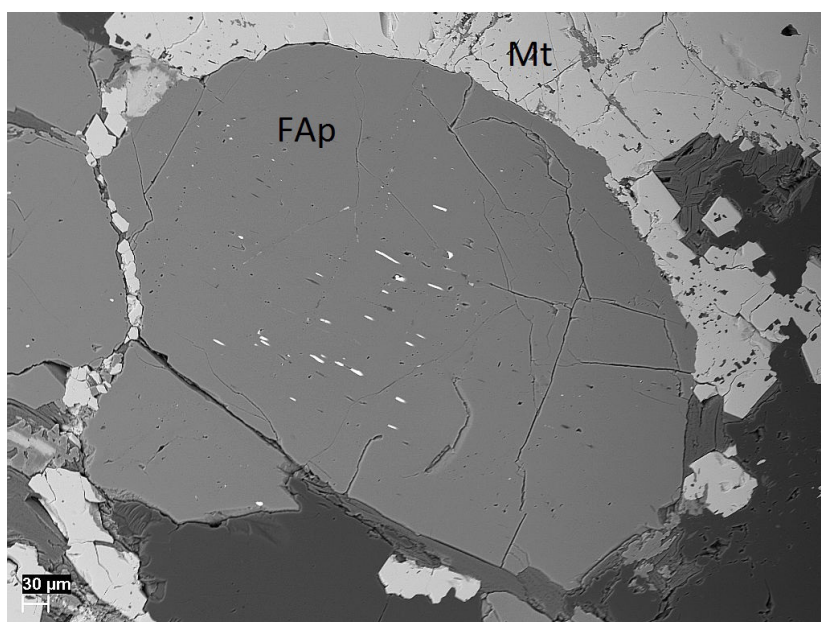
Figure 40. Back-scattered electron (BSE) image showing a rounded-lensoidal fluorapatite (FAP) grain in contact with magnetite (Mt); the fluorapatite exhibits a characteristic texture, containing several BSE-white, epitaxially oriented crystals of monazite-(Ce). The scale bar equals 30 micrometres. Haggruvan, Kopslahyttan area (6694893/ 521413). Photo: Erik Jonsson.
