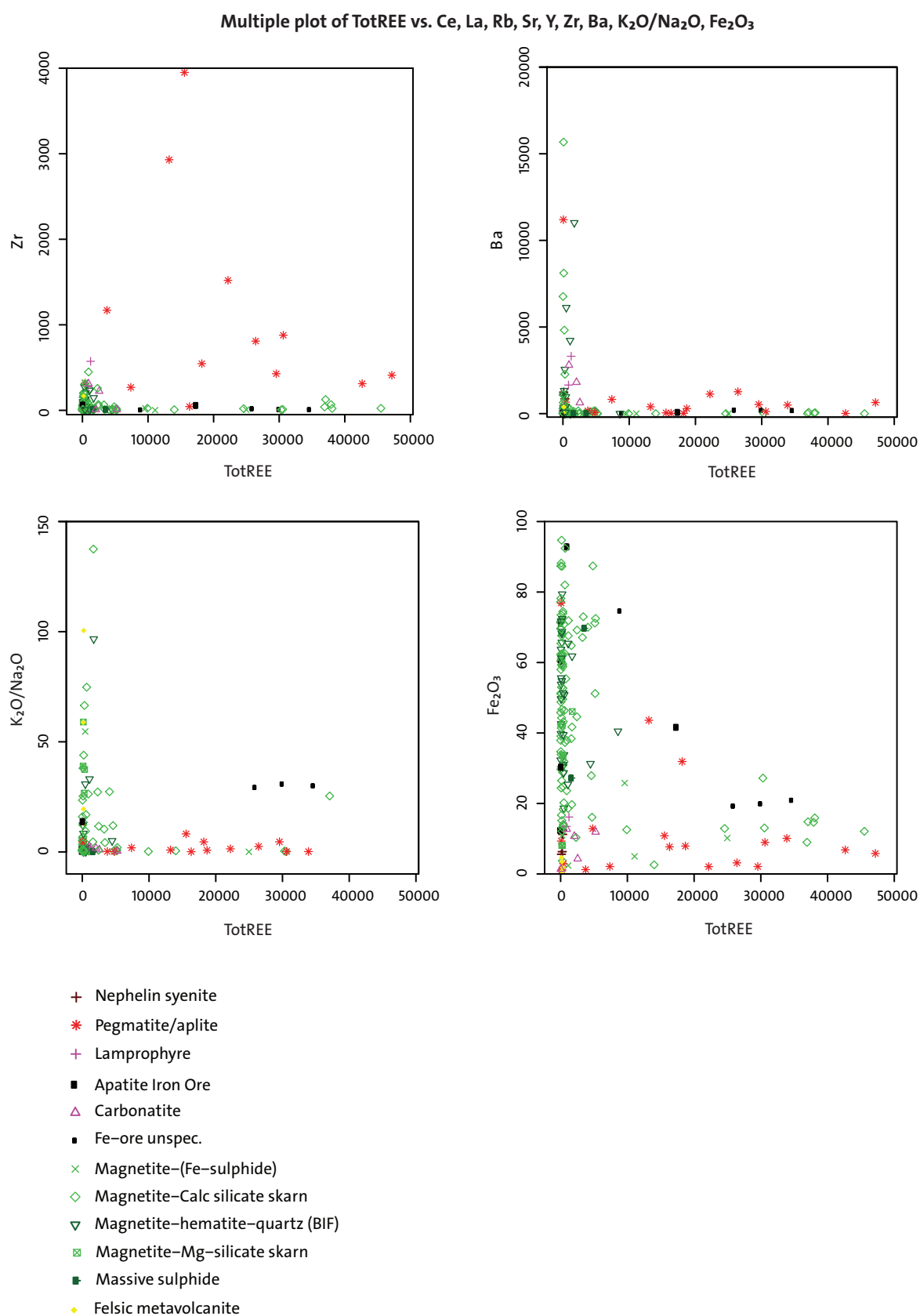
Figure 94. Plots of some elements versus total REE in the samples analysed. Continuation from the previous page.
