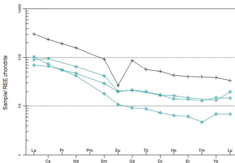
Figure 35. REE plot of host rocks from the Malmberget district (light greenish blue) and Kvikkjokk area (black). Data source: SGU/Lundh 2014.
