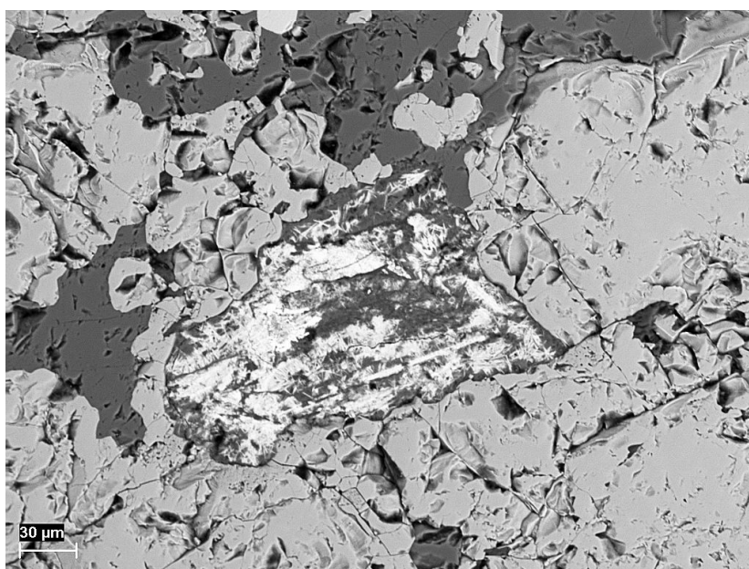
Figure 73. Back-scattered electron (BSE) image showing a heterogeneous aggregate of fine-grained, LREE-bearing silicate and probably fluorocarbonate (both white, centre of image) minerals, in a groundmass of medium grey magnetite and silicates (dark grey). The REE-rich minerals are most likely alteration products, representing a heterogeneous pseudomorph of an unknown primary phase. The scale bar equals 30 micrometres. Gullebo iron mines (6445227/564411). Photo: Erik Jonsson.
