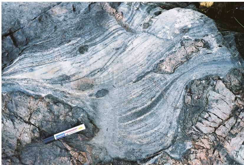
Figure 24. An approximately 50-cm-wide irregular carbonatite dyke incorporating, dissolving and disseminating high-grade fenite (Stornäset). Photo: Johan Söderhielm
