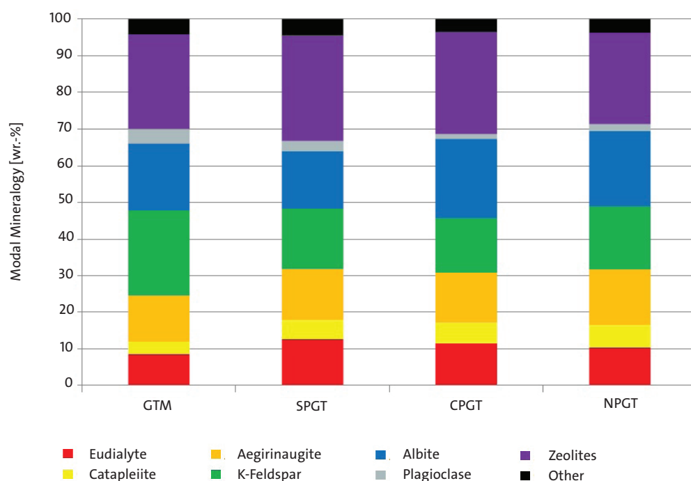
Figure 22. Mineralogical distribution in Norra Kärr mineralised rock types as determined by MLA (Saxon et al. 2015). The abbreviations GTM, SPGT, CPGT, and NPGT are explained in the text and Fig. 20.
