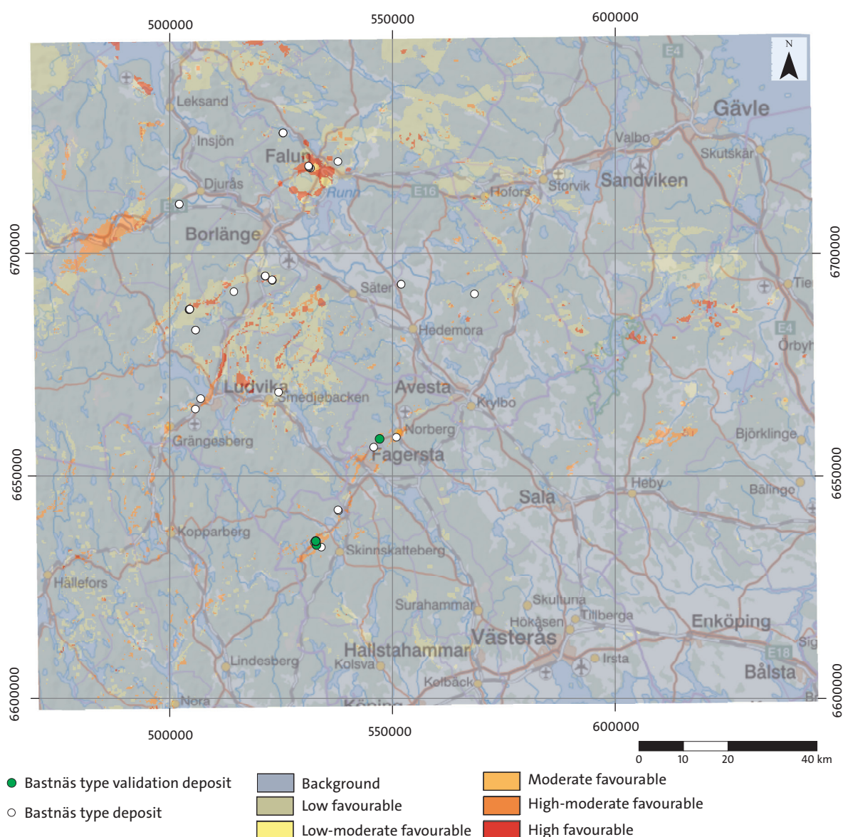
Figure 104. Relative degree of prospectivity for skarn-hosted REE mineralisation in Bergslagen.
