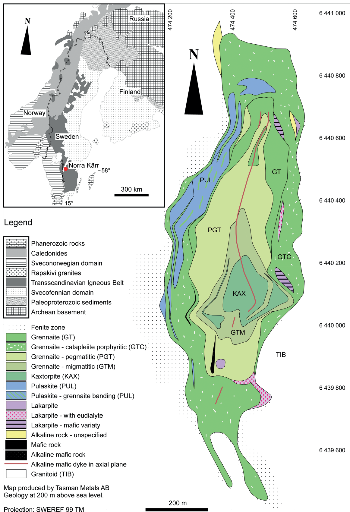
Figure 20. Bedrock geology of the Norra Kärr complex, including unit classification, courtesy of Tasman Metals/Leading Edge Materials (source: Saxon et al. 2015)
