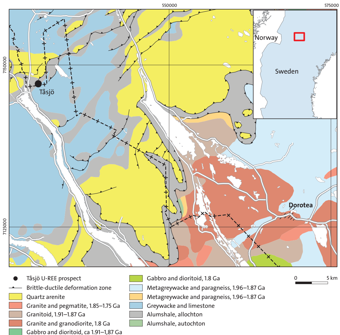
Figure 87. Simplified bedrock geology map showing the location of the Tåsjö U-REE prospect at the border between Västerbotten and Jämtland counties.
