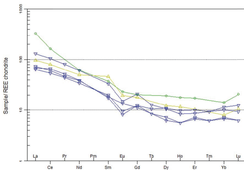
Figure 34. REE plot of host rocks from the northern districts; Kirunavaara (green); Svappaavaara (yellow); Vähävaara/Masugnsbyn (blue). Most of the samples display a distinct Eu trough and a relative enrichment in LREE compared to the HREE. All samples are normalised to chondrite values from Boynton (1984). Data source: SGU/Lundh 2014.
