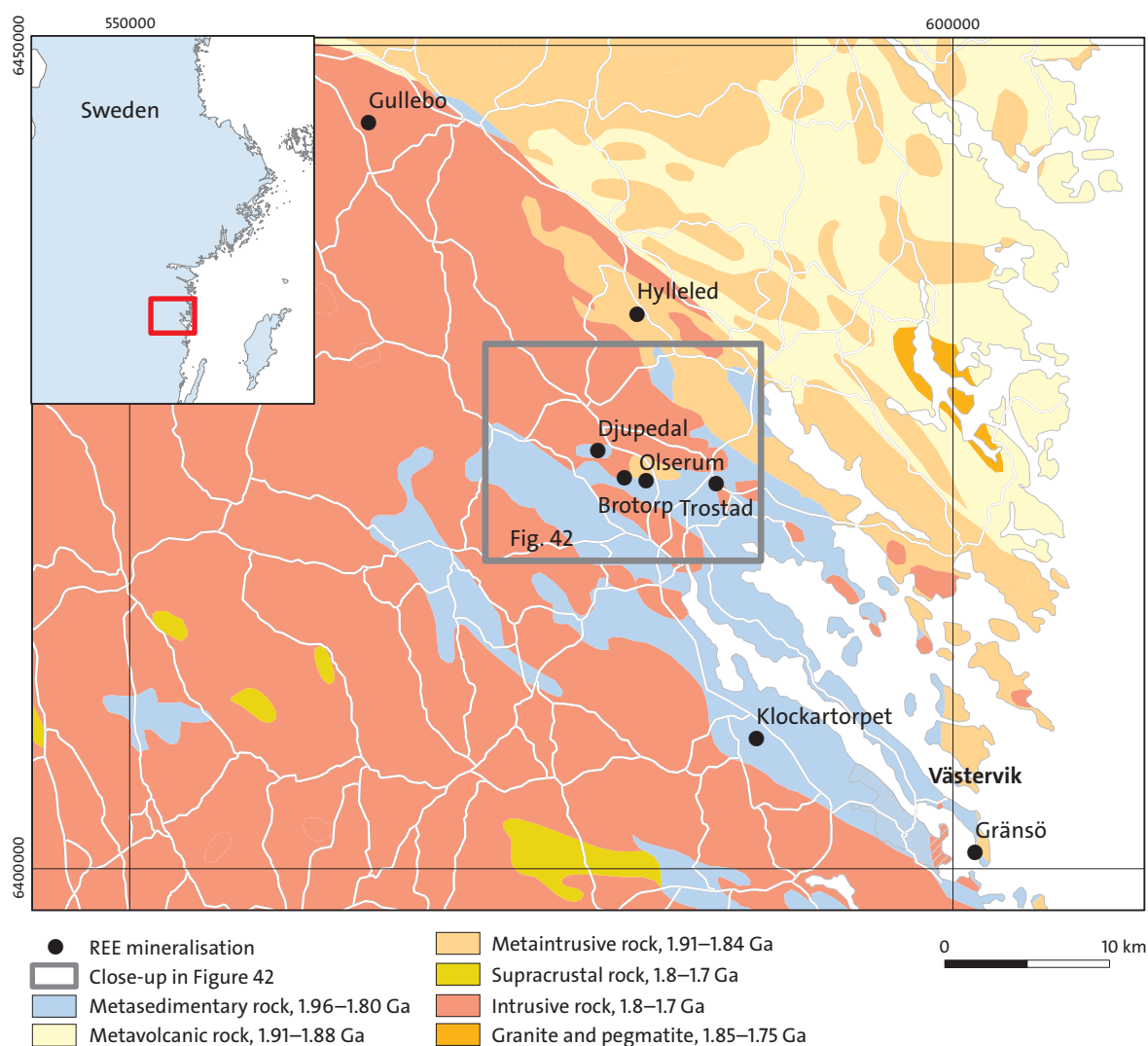
Figure 41. Simplified bedrock geological map showing the locations of Olserum and other REE mineralisations in this area.
