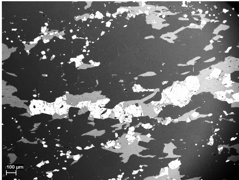
Figure 84. Back-scattered electron (BSE) image showing an overview of “heavy mineral bands” in a quartzitic rock from Gränsö Södra: the predominant white mineral is magnetite; smaller white(r) grains are monazite, xenotime and U-rich phases. The medium grey mineral directly associated with magnetite is a biotitic mica. The dark grey/black groundmass is quartz. Photo: Erik Jonsson.
