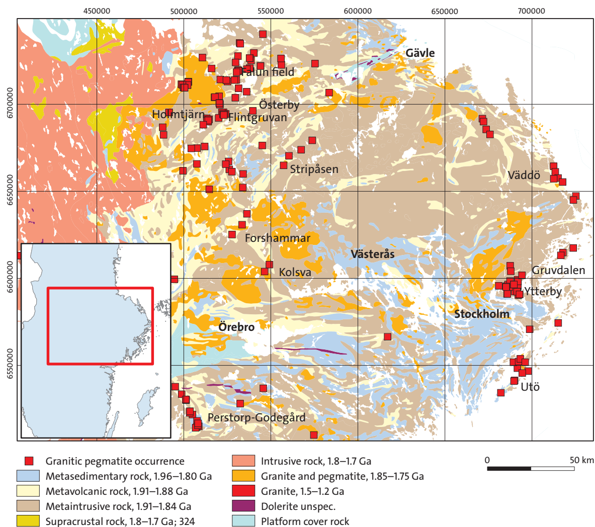
Figure 9. Simplified bedrock geology map showing locations of quarried granitic pegmatites in south-central Sweden, essentially within the Bergslagen ore province; REE-enriched occurrences or clusters mentioned in the text are named.
