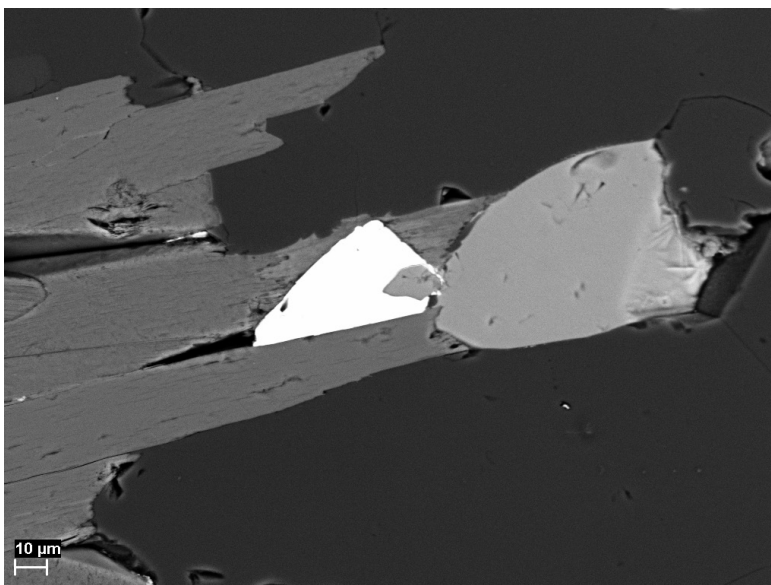
Figure 86. Back-scattered electron (BSE) image of REE mineralisation at Gränsö Södra: a subhedral crystal of xenotime-(Y) (white), enclosed in biotite (dark grey, platy), in contact with subhedral to anhedral fluorapatite (light grey) enclosed in quartz (darkest grey/black). Photo: Erik Jonsson.
