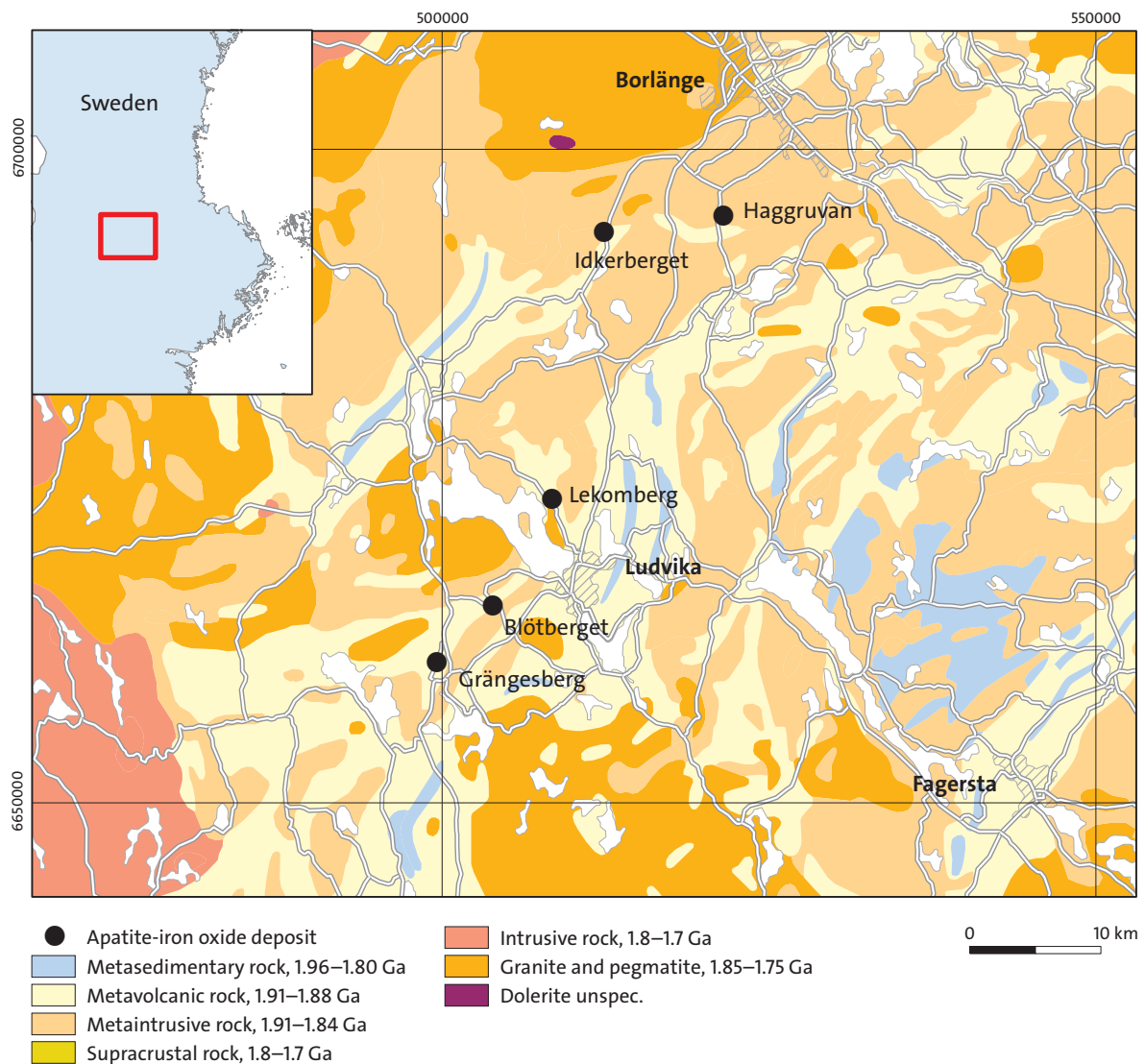
Figure 36. Simplified bedrock geology map of a part of northwestern Bergslagen, showing the locations of the major apatite-iron oxide deposits (and one minor deposit – Haggruvan).
