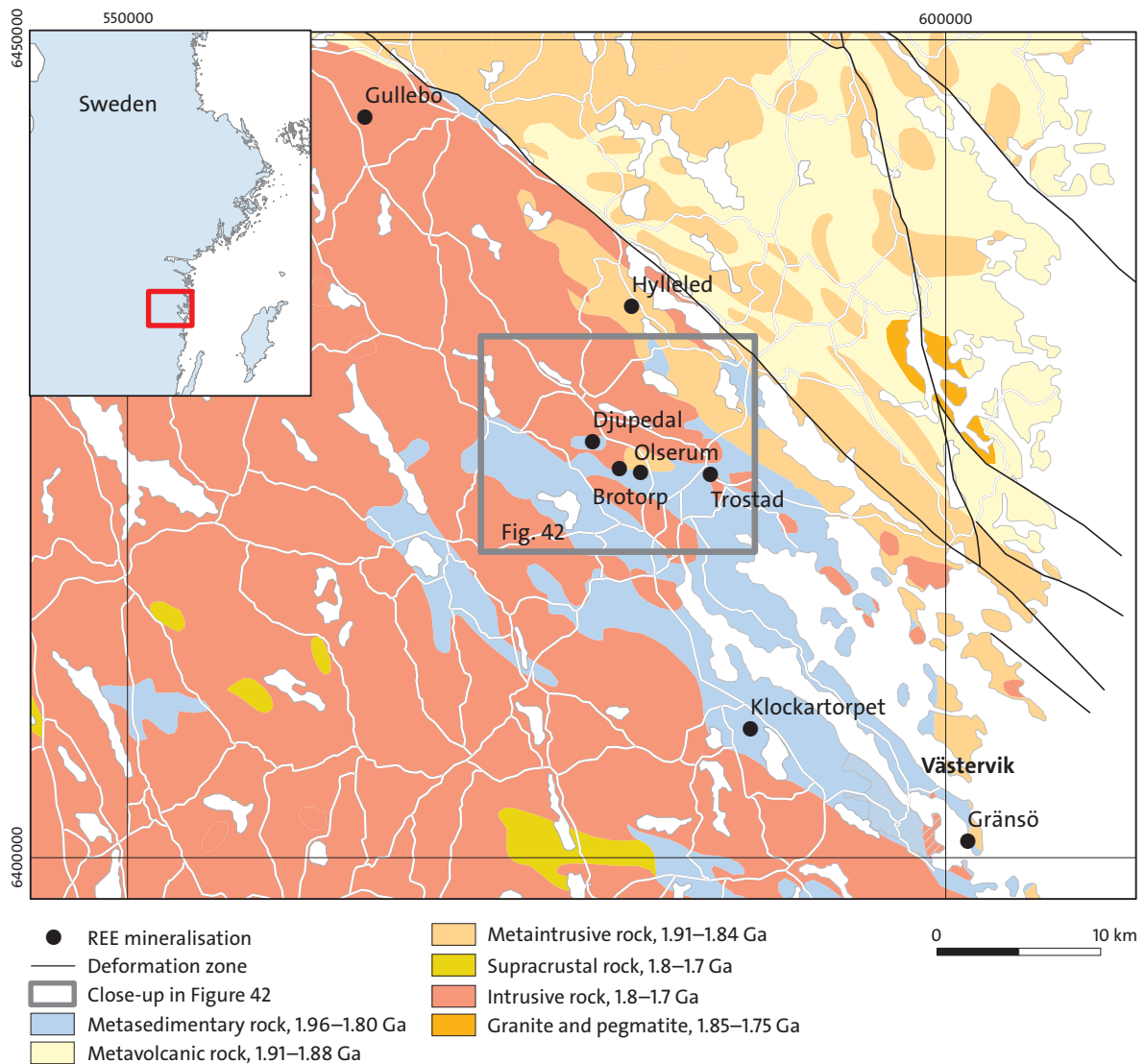
Figure 72. Simplified bedrock geology map showing the locations of the REE-mineralised iron oxide deposits at Gullebo and Hylleled, and their spatial relationship to the mineralisations in the Västervik area (inset rectangle corresponds to Fig. 42 in this chapter).
