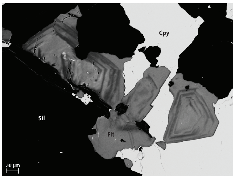
Figure 79. Back-scattered electron (BSE) image showing distinctly zoned subhedral crystals of REE-bearing fluorite (Flt; grey shades) in contact with a later-formed chalcopyrite infilling (Cpy; white) in a silicate groundmass (Sil; black). The scale bar equals 30 micrometres. Bredåsen (6689355/ 661045). Photo: Erik Jonsson.
