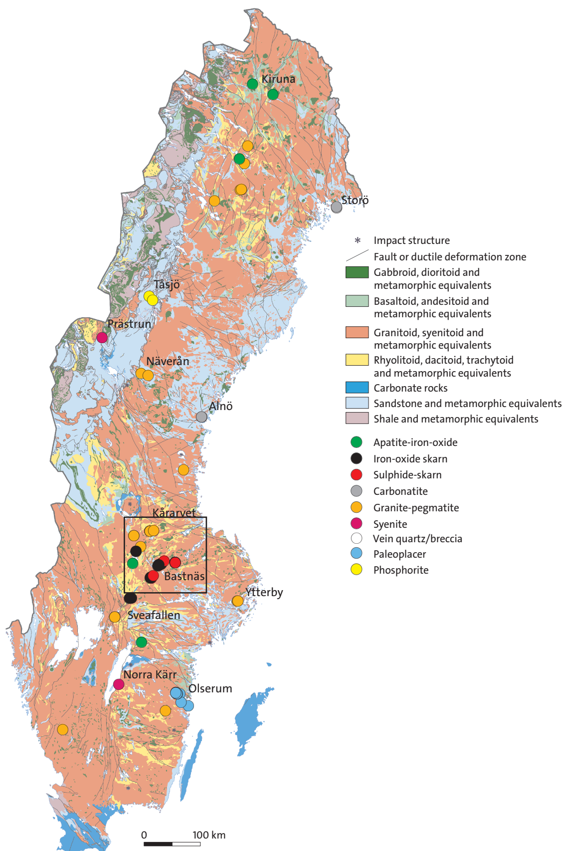
Figure 103. Simplified geological map and classified REE mineralisations in Sweden. The study area is marked by the black rectangle. (Source: SGU, Mineral resources database)
