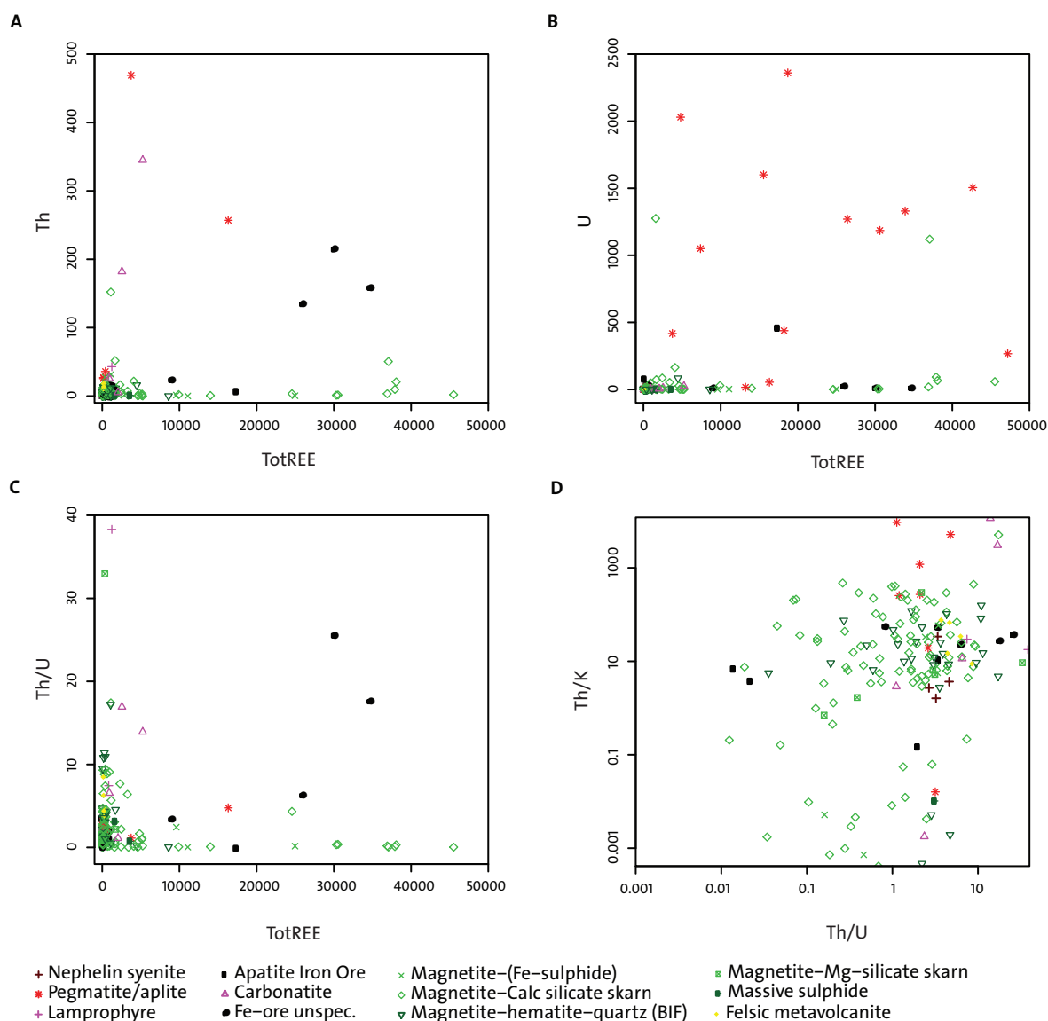
Figure 93. Bivariate plots of A. Th vs total REE; B. U vs total REE; C. Th/U vs total REE; and D. log Th/K ratio vs log Th/U ratio for the samples analysed. Symbols as in Fig. 92.
