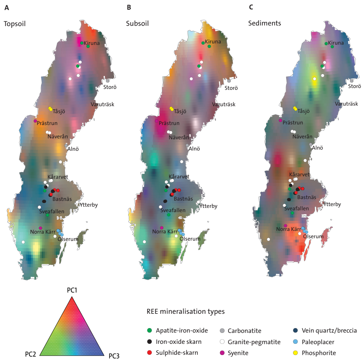
Figure 88. Colour composite images of PC1 (red), PC2 (green) and PC3 (blue) of individual Swedish FOREGS datasets: A. topsoils; B. subsoils; C. stream sediments.
