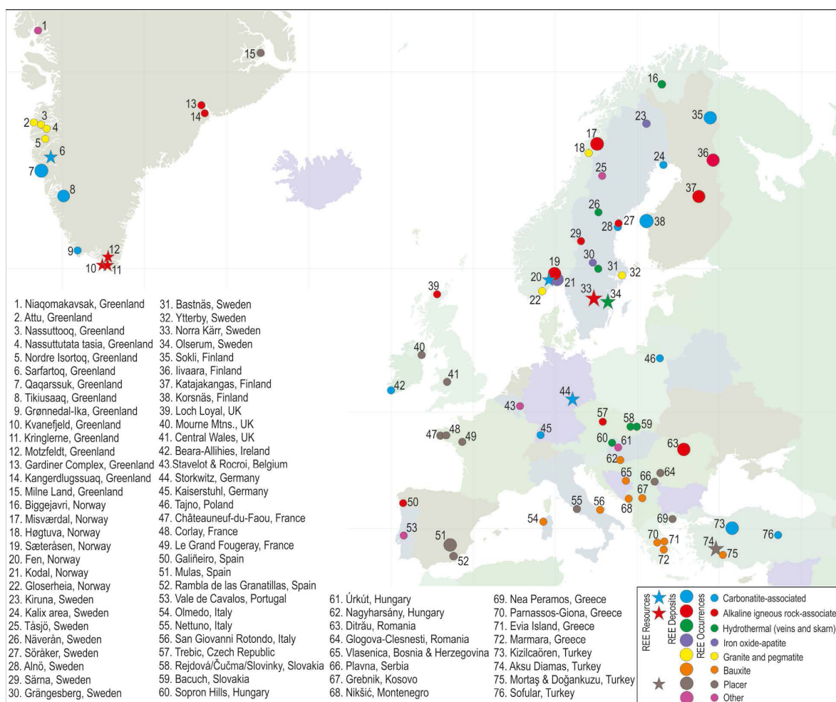
Figure 1. Map of European REE mineral deposits and occurrences in Europe (Source: www.eurare.org ).
