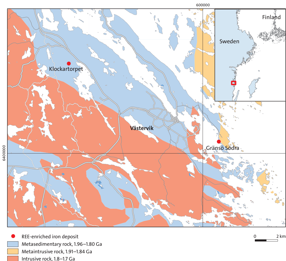
Figure 81. Simplified bedrock geology map showing the location of the Gränsö Södra and Klockartorpet mineralisations in the Västervik area.
