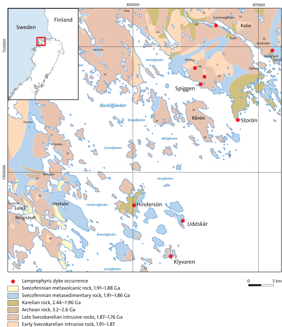
Figure 26. Simplified bedrock geology map showing locations of the Luleå–Kalix section of the northern Swedish coast, including known locations of lamprophyric dykes.
