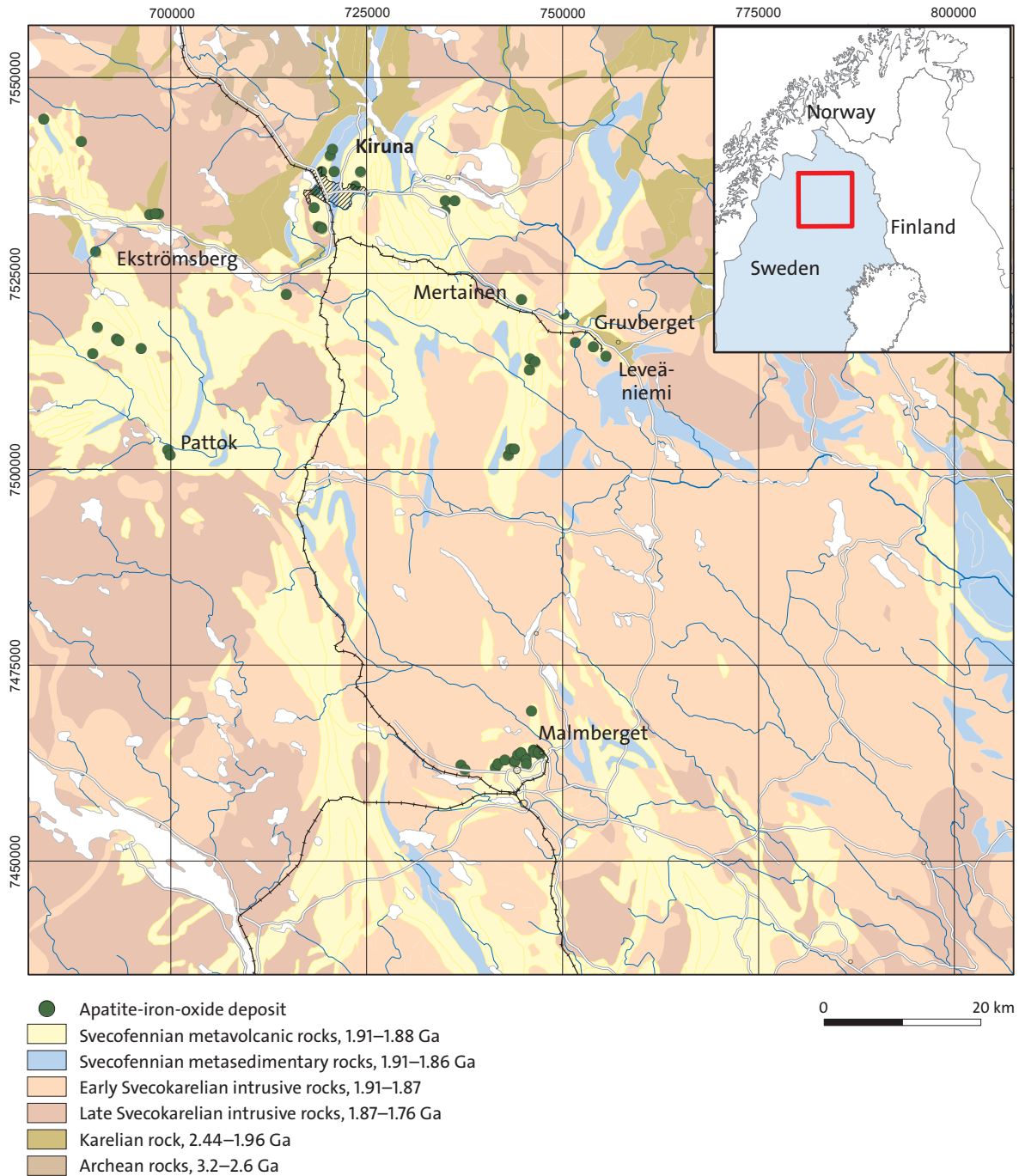
Figure 32. Simplified bedrock geological map of central northern Norrbotten, showing the locations of the Kiruna and Malmberget mines and other significant apatite-iron oxide deposits.
