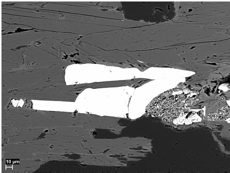
Figure 85. Back-scattered electron (BSE) image showing subhedral monazite-(Ce) crystals (white) intergrown in biotitic mica, with associated partly altered iron oxides to the right in the image. Photo: Erik Jonsson..
