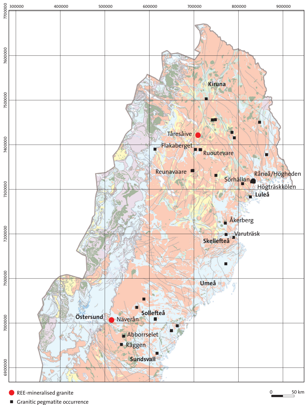
Figure 12. Simplified bedrock geology map showing locations of quarried granitic pegmatites and REE-mineralised granitoids in northern Sweden; occurrences or clusters mentioned in the text are named.
