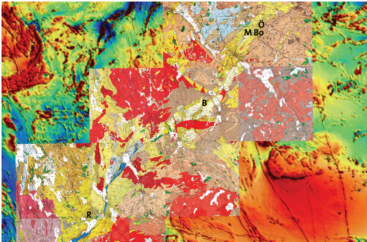
Figure 97. The approximate extent of the REE line on bedrock maps (scale 1:50 000) published by the Geological Survey of Sweden and a background of the aeromagnetic anomaly map. The extent of each bedrock map is 25 x 25 kilometres, north is up. R denotes Rödbergsgruvan, B – Bastnäs, M – Malmkärr, Bo – Bojmossfältet and Ö – Östanmossa.
