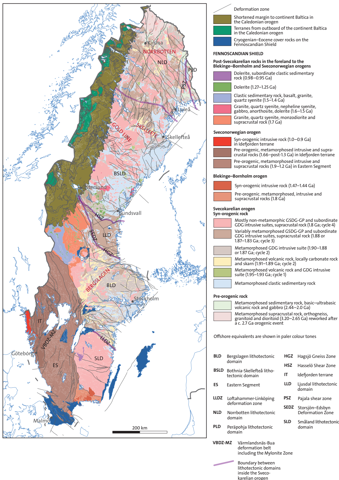
Figure 2. Simplified bedrock geological map of Sweden (modified from Stephens & Weihed 2013). The image was generated using the 1:1 million national bedrock database for Sweden at the Geological Survey of Sweden (SGU). GDG = granitoid-dioritoid-gabbroid, GP = granite-pegmatite, GSDG = granite-syenitoid-dioritoid-gabbroid. The position of the major ore districts (Bergslagen, Caledonides, Skellefte, Norrbotten) and the “Gold Line” of the Sveco-Karelian orogen are indicated.
