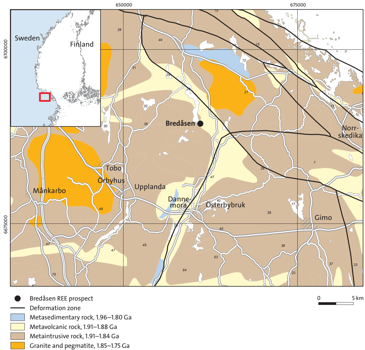
Figure 77. Simplified bedrock geology map showing the location of the Bredåsen mineralisation in northeastern Bergslagen.
