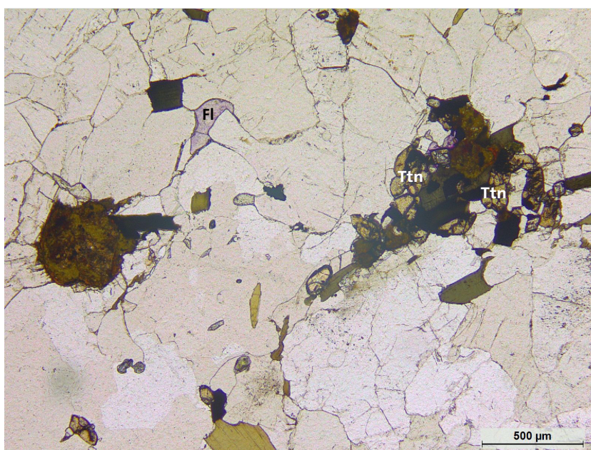
Figure 14. Transmitted polarised light image of a representative polished thin section of the RA-granite sampled for the bedrock quality study of Eliasson et al. Aggregates of titanite (Ttn), zircon, chlorite/biotite and opaque oxide minerals occur in a fluorite-bearing (Fl) quartz-feldspar groundmass. Photo: Thomas Eliasson.
