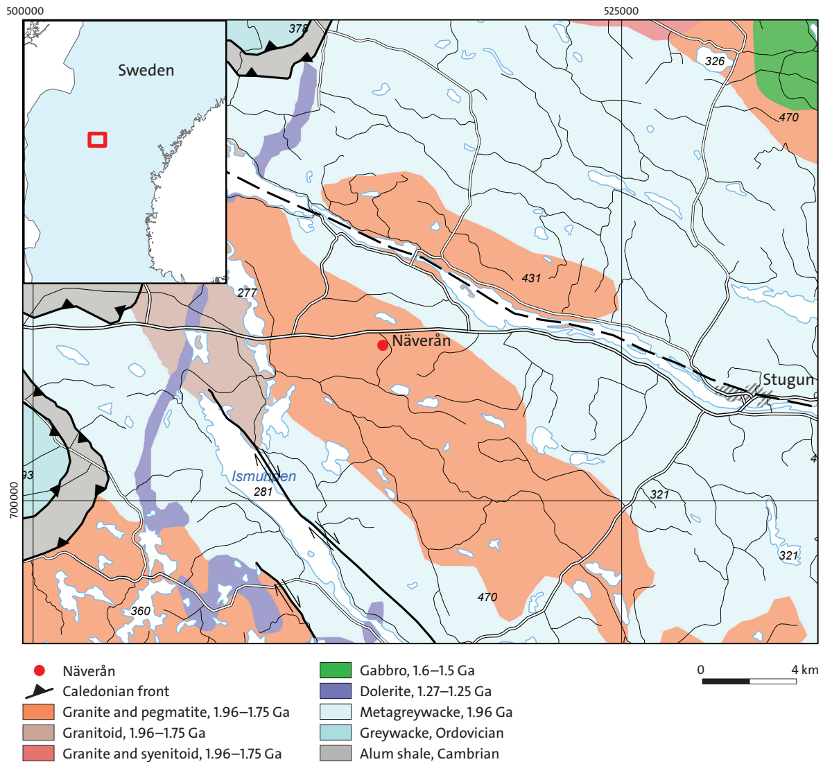
Figure 15. Simplified bedrock geology map showing the location of the Näverån mineralisation (7006810/ 515025), a few kilometres east of the Caledonian front.
