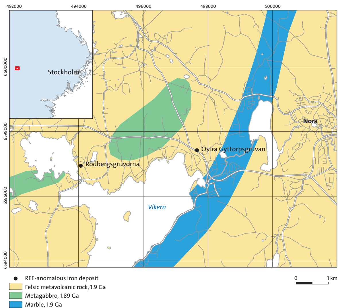
Figure 61. Simplified bedrock geology map showing locations of known REE mineralisations in the Nora area, in the southwestern part of the REE line.
