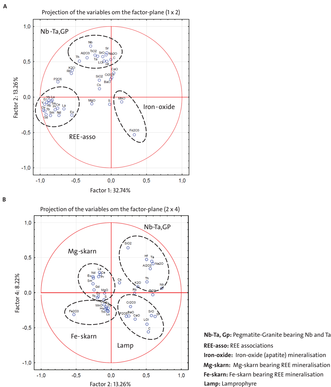
Figure 96. Plots of A. PC1 vs PC2; and B. PC2 vs PC4.
