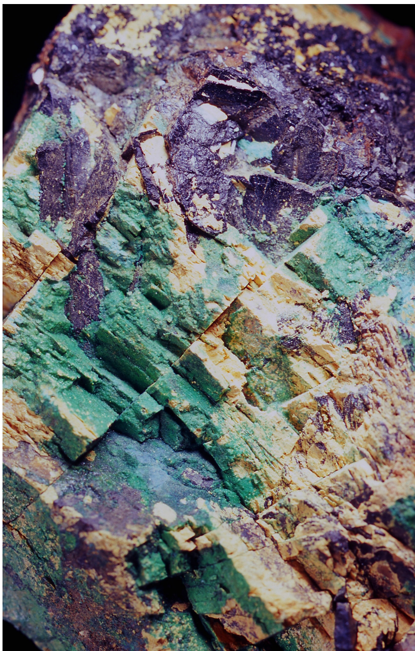
Figure 52. Coarse bastnäsité-(Ce) occurring as a radial crystal aggregate has been extensively replaced by dullish, light yellow hâleniusite-(La), and also covered by precipitates of a green secondary copper mineral, probably brochantite. Platy black crystals of ferriallanite-(Ce) border and are partly intergrown with the (former) bastnäsité in the upper part of the image. Nya Bastnäs mines. Specimen from the collection of the Swedish Museum of Natural History (Stockholm). Image width approximately 2.5 cm. Photo: Erik Jonsson.
