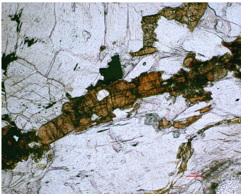
Figure 66. Brown, allanite-like mineral as subhedral crystals or fissure-fillings in skarn at Mörkens #4, Knutsbo area. Photomicrograph in transmitted plane-polarised light. The scale bar equals 100 micrometres. Photo: Per Nysten.
