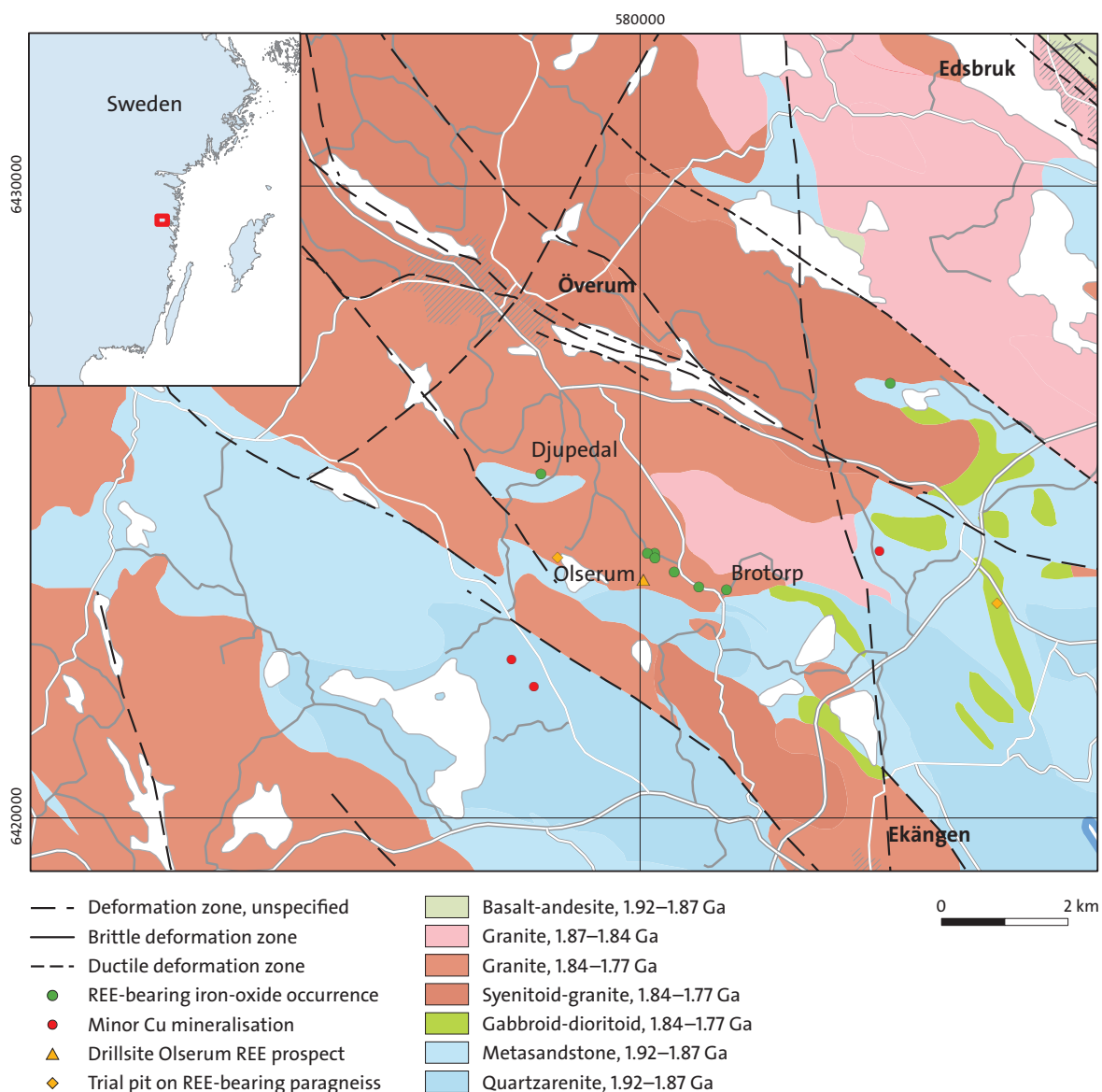
Figure 42. Bedrock geological map of the Olserum area with known mineralisations marked; the most important are named (Brotorp is also known as Källhagen).
