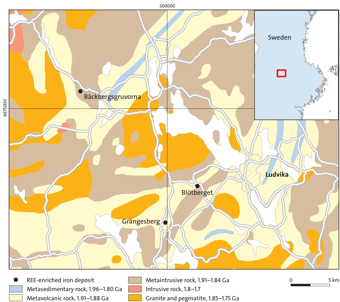
Figure 75. Simplified bedrock geology map showing the location of the REE-mineralised iron oxide mines Bäckbergsgruvorna, in the northwestern part of the Bergslagen province. The locations of the Blötberget and Grängesberg REE-enriched, major apatite-iron oxide deposits are also shown.
