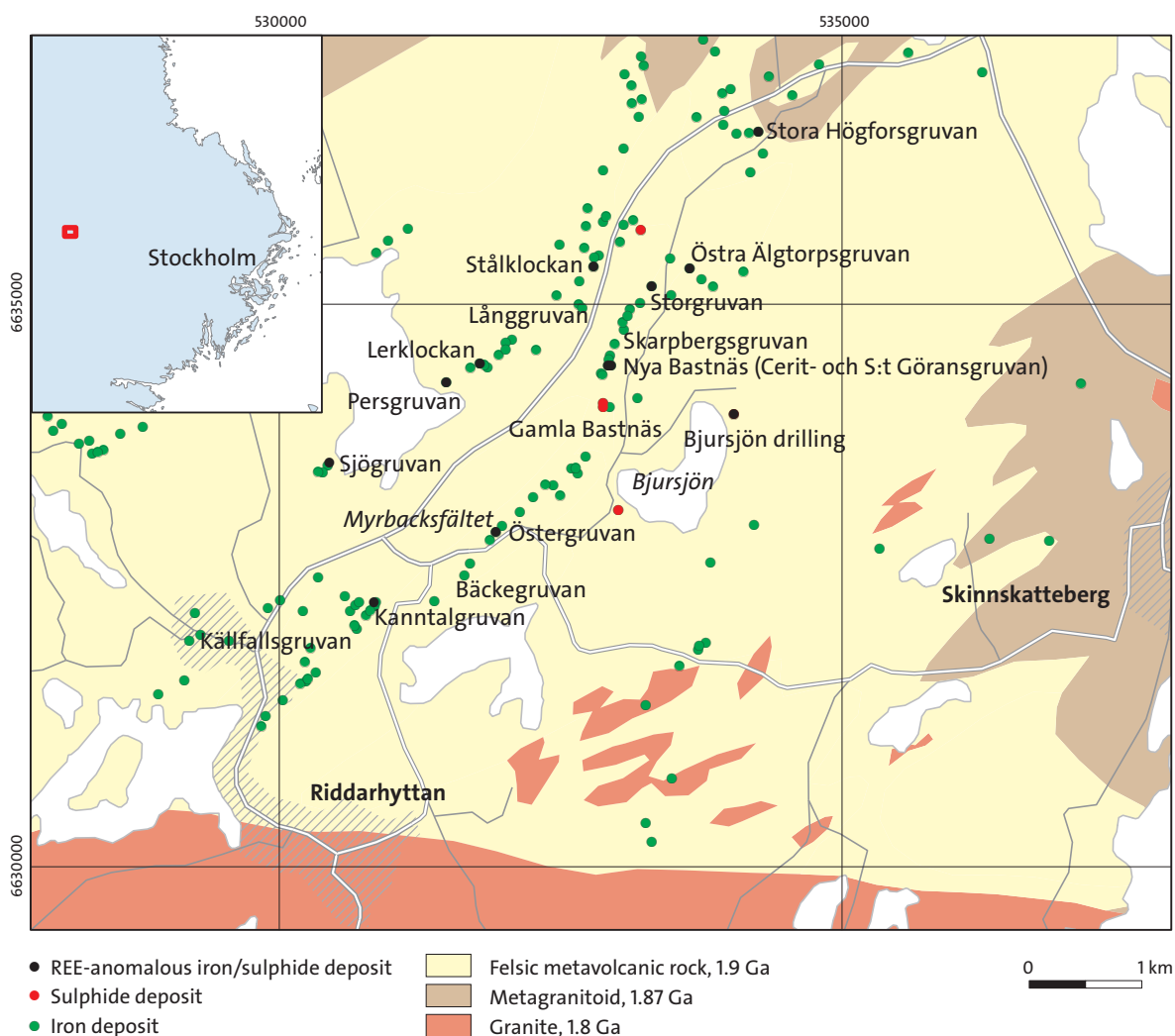
Figure 50. Simplified bedrock geology map showing locations of mines in the Riddarhyttan field, central part of the REE line, highlighting those with REE enrichment.
