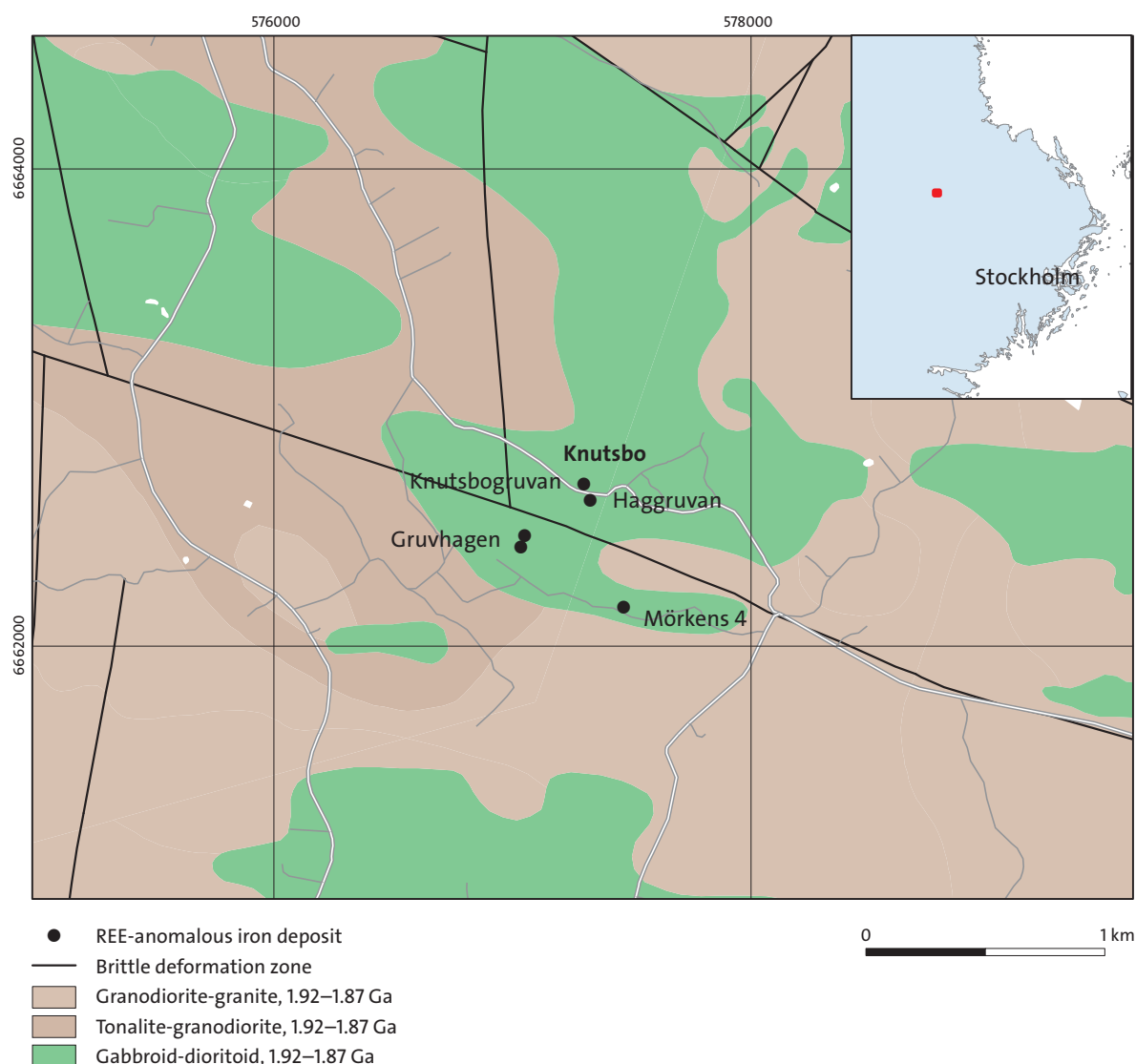
Figure 65. Simplified bedrock geology map showing locations of mines with REE mineralisation in the Knutsbo area, northeasternmost part of the REE line.
