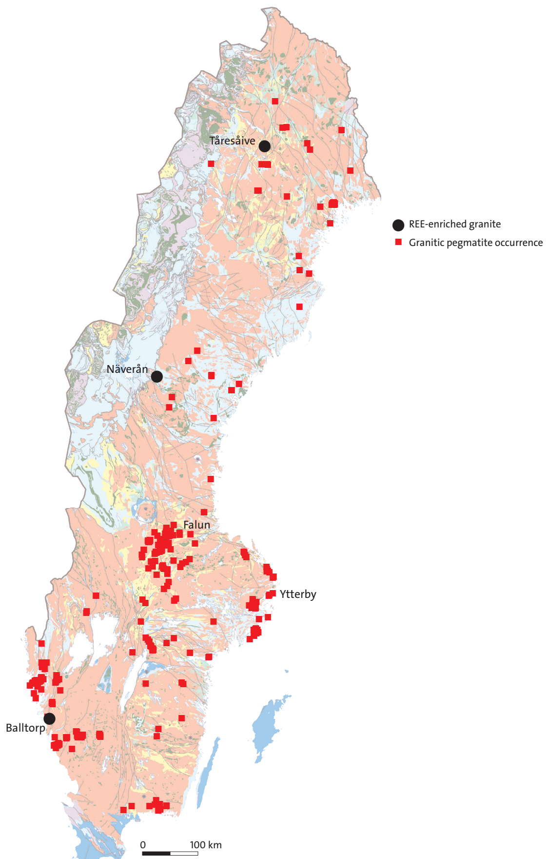
Figure 4. Major granitic pegmatite quarries and occurrences of REE-mineralised granitoids in Sweden.
