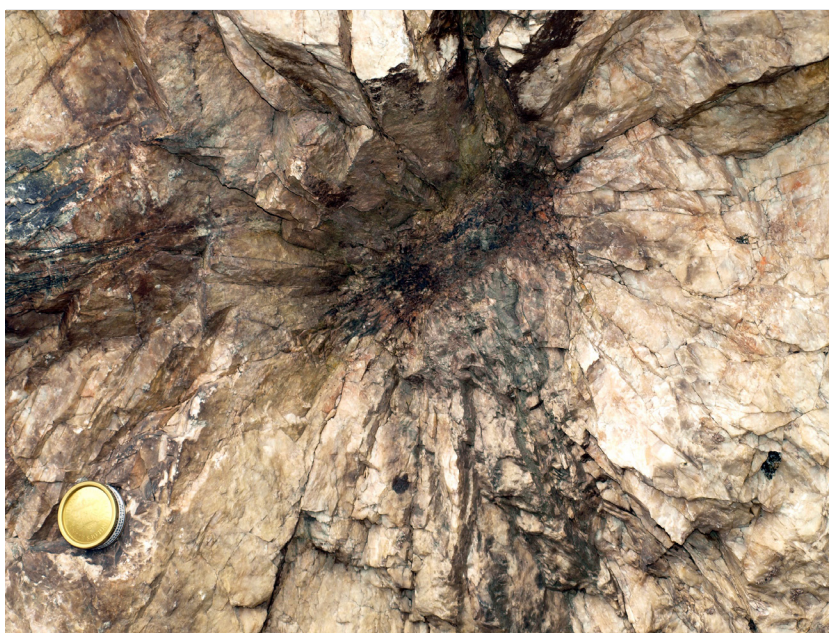
Figure 6. Partly altered metamict and heterogeneous aggregate of highly radioactive REE minerals in the western wall of the uppermost part of the Ytterby pegmatite quarry, near Vaxholm (6592332/690226). The radial fracture pattern in the feldspar-dominated rock surrounding the large, brownish to black radioactive aggregate can be readily seen. The snus box for scale is 70 mm in diameter. Photo: Erik Jonsson.
