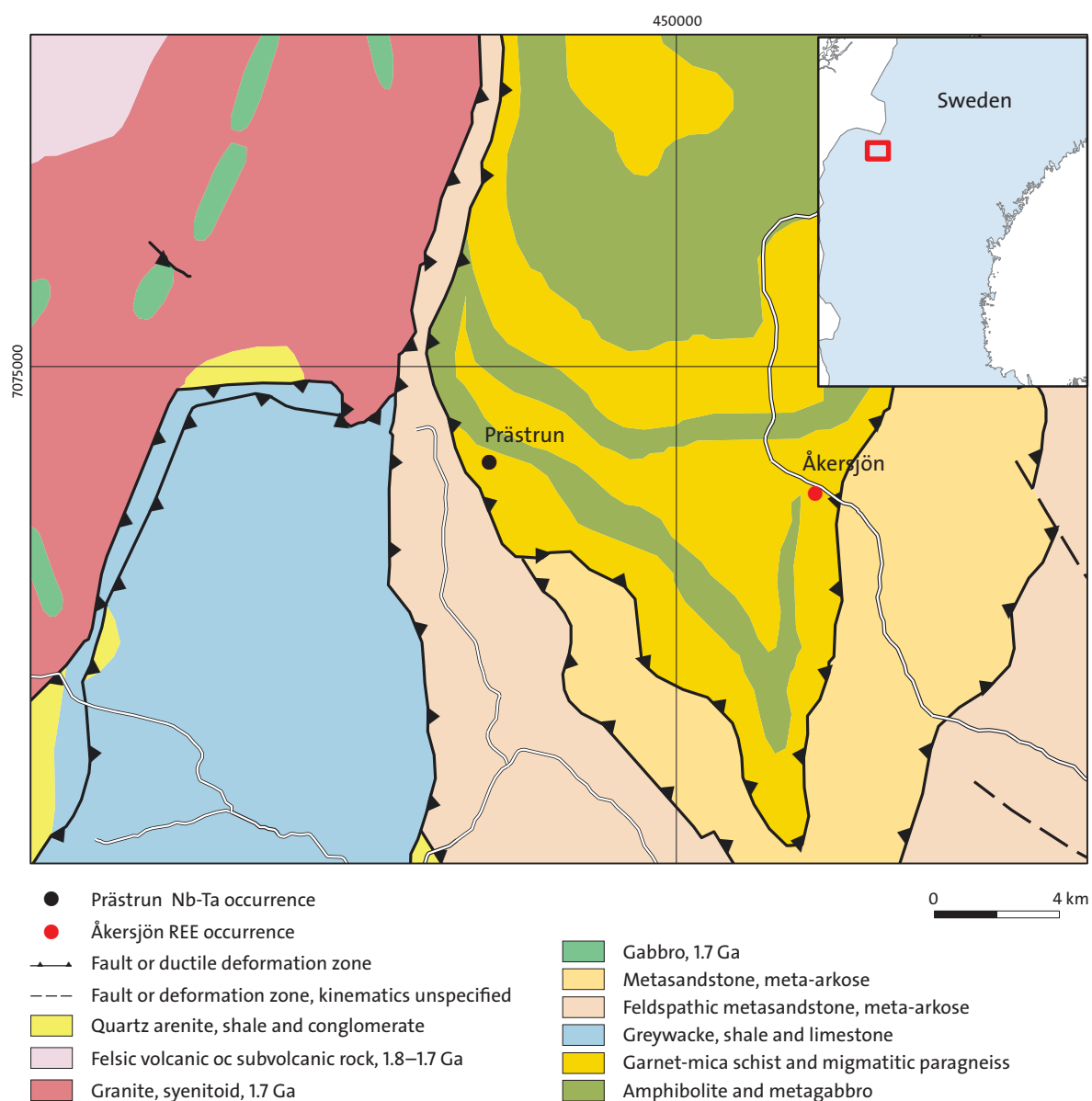
Figure 28. Simplified bedrock geology map showing locations of Åkersjön (7071002/454407) and the Prästrun (7071939/443926) mineralisations in the central Swedish Caledonides.
