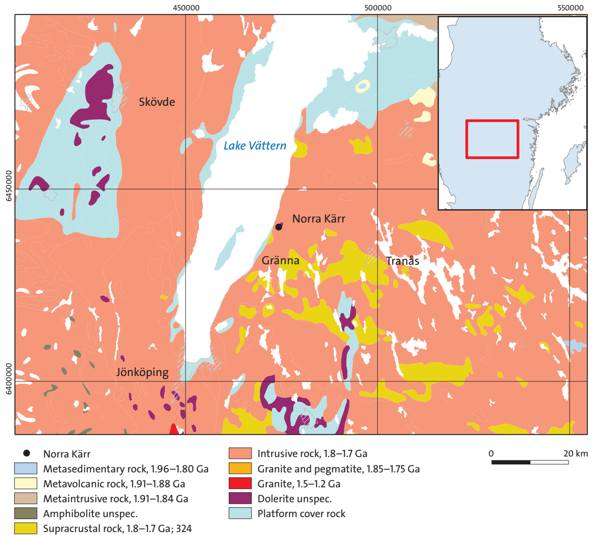
Figure 19. Simplified bedrock map showing the location of the REE-mineralised Norra Kärr nepheline syenite complex (6440266/ 474525) east of Lake Vättern, southern Sweden.
