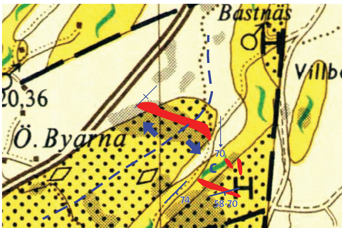
Figure 99. The geology of the Bastnäs area. The background is the bedrock map by Ambros (1983). Red areas are mapped outcrops and blue symbols are additional structural data from this study. C denotes cordierite-bearing. The view is approximately 1.5 km wide. N is up.
