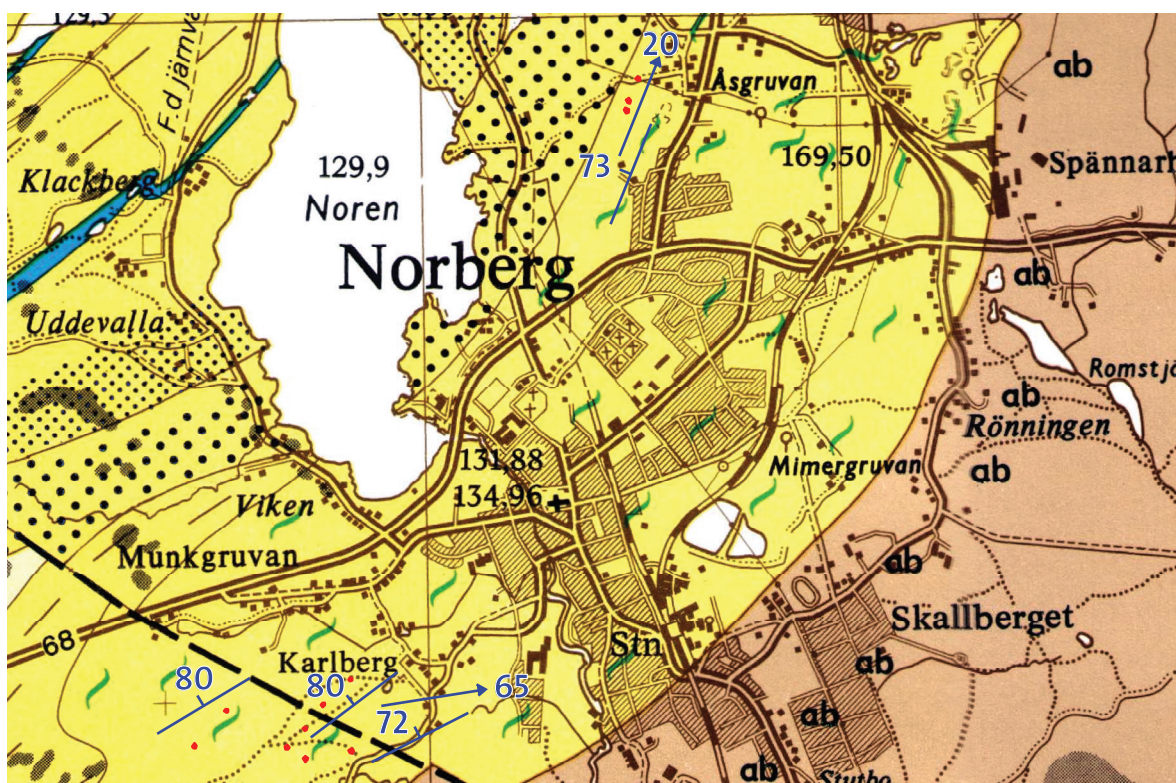
Figure 101. Geology of the Norberg area. The background is the bedrock map by Ambros (1988). Small, red dots denote outcrops investigated in this study. Additional structural measurements in blue. The view is approximately 4.5 km wide. N is up.
