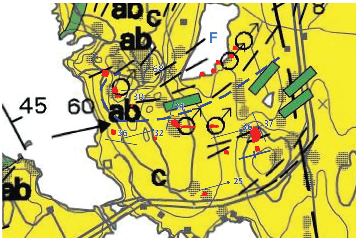
Figure 98. The area around Stora Rödbergsgruvan. F denotes lake Fogdhyttetjärnen. The background bedrock map is by Stephens (1998). The width of view is approximately 1.5 km, N is up. Red dots are observed outcrops and pits in this study. The blue structural symbols and broken line are measurements and interpretation by this study.
