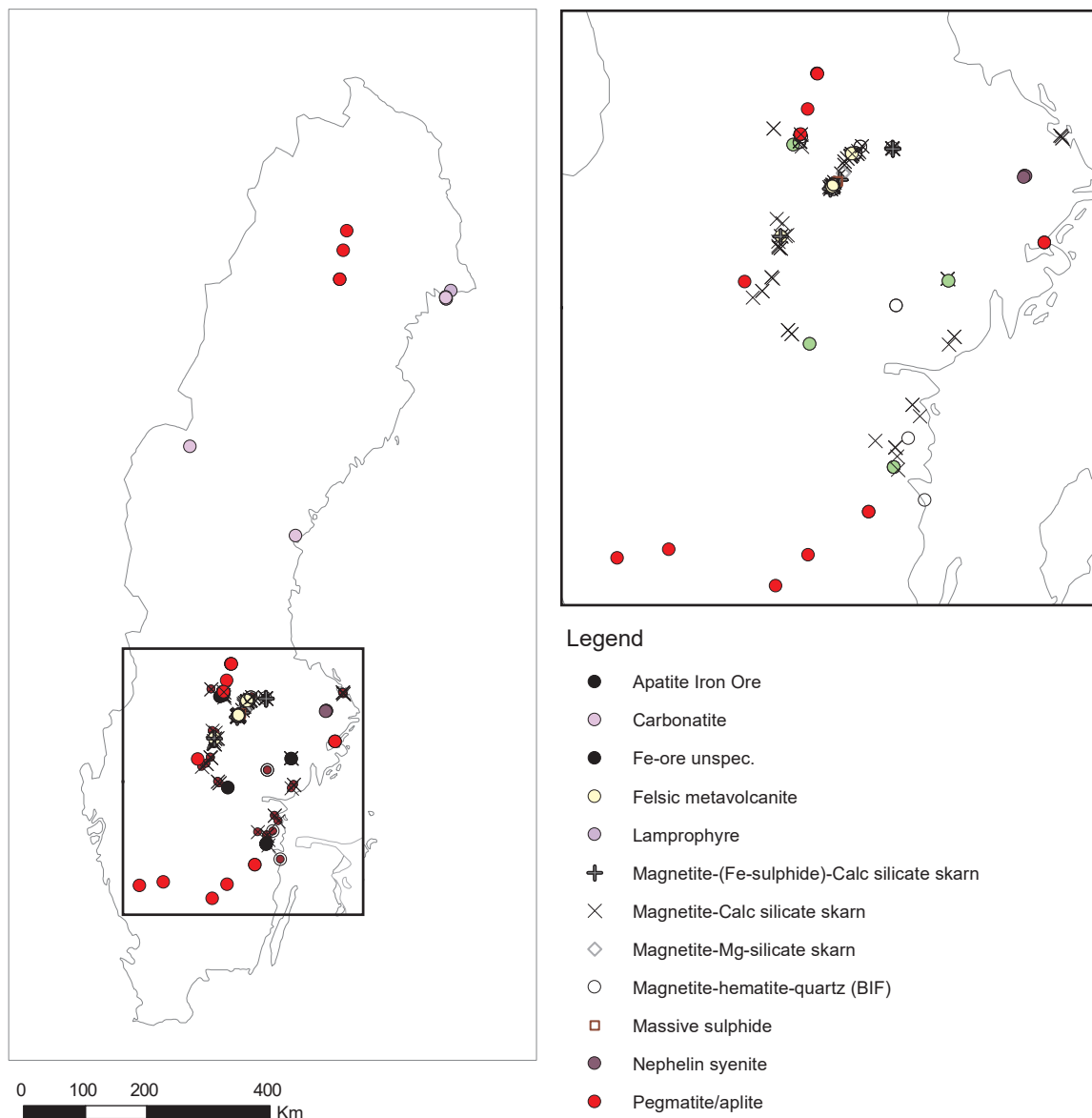
Figure 91. Simplified location map of samples in the EURARE project.
