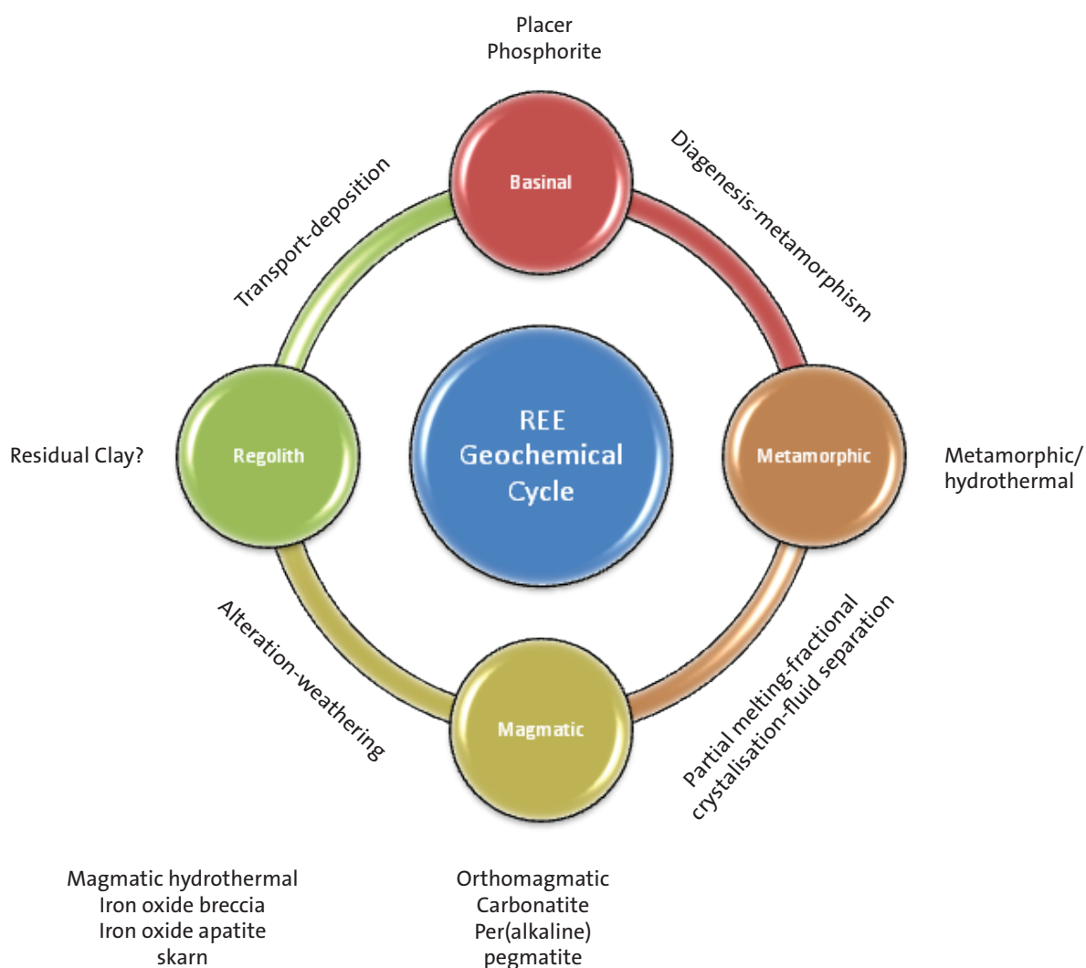
Figure 90. Geochemical cycle for rare earth elements (only REE mineralisations in Sweden have been considered here; modified from Hoatson et al. 2011). Alkaline and carbonatitic melts, produced by the partial melting of mantle, transport rare earth elements from the mantle into the crust. Granites that are produced from the partial melting of crustal material are also enriched in rare earth elements (less enriched than alkaline and carbonatitic melts).
