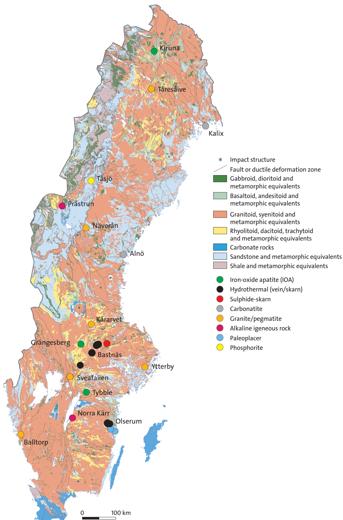
Figure 3. Simplified map of the bedrock geology of Sweden, with a selection of REE deposits, prospects and occurrences.
