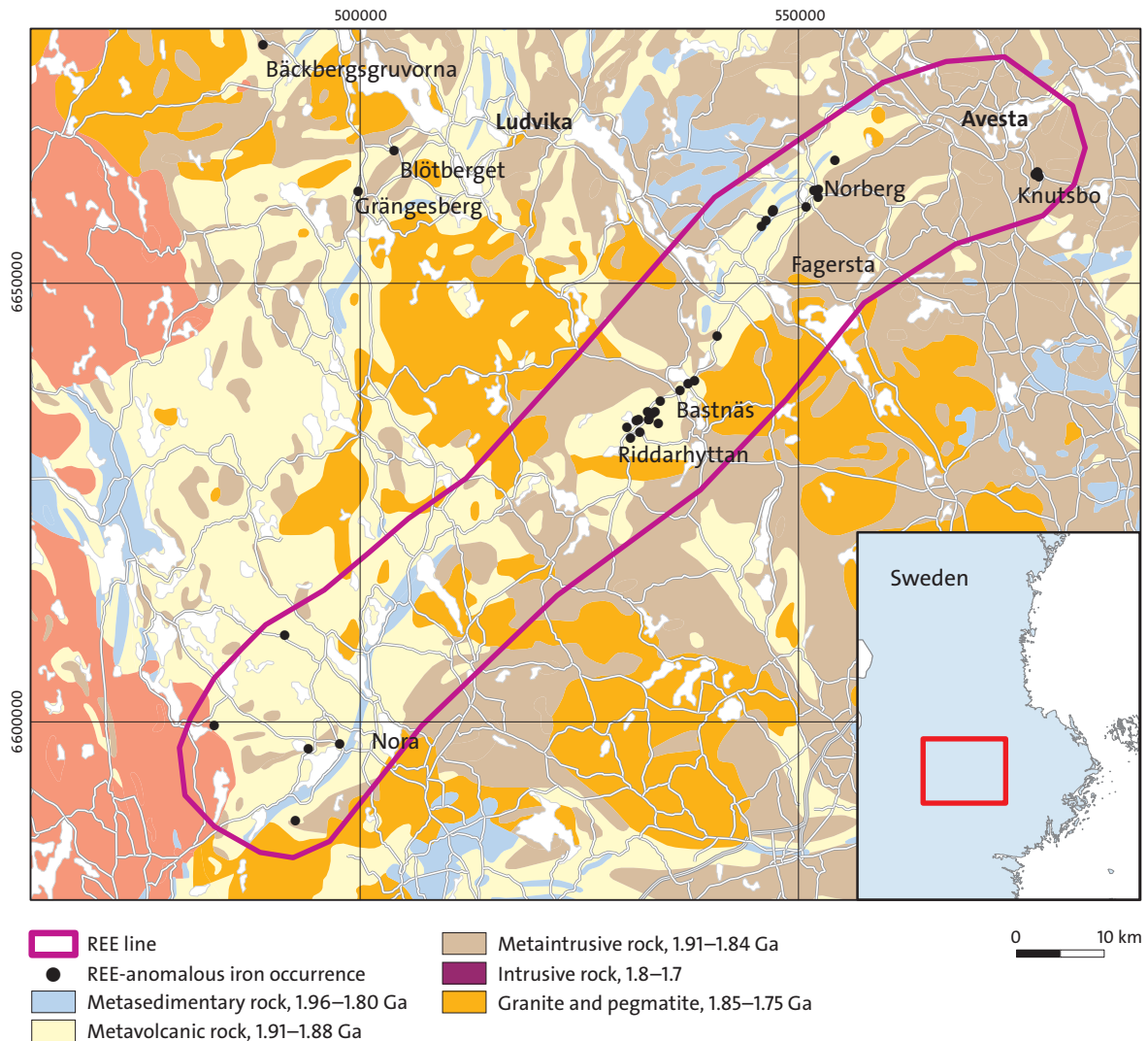
Figure 46. Simplified bedrock geology map showing the main locations or clusters of REE-rich iron-skarn deposits in the REE line.
