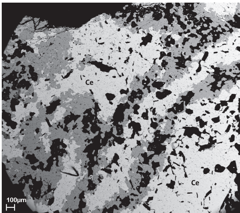
Figure 49. Back-scattered electron (BSE) image of a section from the folded and recrystallised REE silicate bands in the banded iron formation mined at Högfors. Small-scale folding can be seen in the alternating bands of cerite-(Ce) (light grey/white) and a darker grey västmanlandite-like mineral, most likely the unnamed Fe analogue of västmanlandite-(Ce). Black represents silicates, mostly amphibole. Photo: Erik Jonsson.
