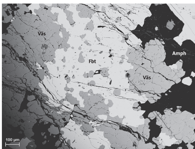
Figure 56. Back-scattered electron (BSE) image of the REE-rich mineralisation from Stålklockan, showing the predominant intergrowth of a BSE-white fluorbritholite-(Ce) (Fbt) with a västmanlandite-like mineral (Väs; medium grey), together with skarn amphibole (Amph; black). The fine-grained and recrystallised texture of the REE silicates is apparent. Photo: Erik Jonsson.
