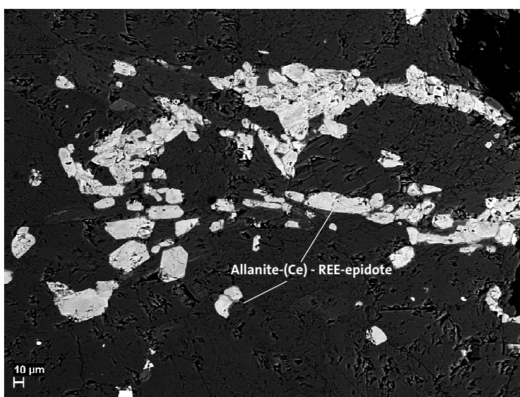
Figure 76. Back-scattered electron (BSE) image showing fine-grained crystals and aggregates of euhedral to subhedral REE epidote-allanite-(Ce) in a skarn silicate groundmass. The variable (mottled) grey scale of the crystals is primarily due to variations in REE content. The scale bar equals 10 micrometres. Bäckbergsgruvorna. Photo: Erik Jonsson.
