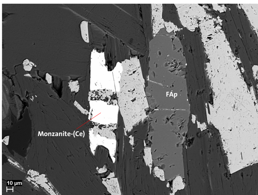
Figure 70. Back-scattered electron (BSE) image showing a silicate-bearing (darkest grey to black) magnetite (lightest grey) ore, with magnetite in part intergrown with blocky monazite-(Ce) (white), fluorapatite (REE-free; medium grey), locally hosting fine-grained fracture fillings and aggregates of REE-bearing phases). The scale bar equals 10 micrometres. Bojgruvan (6551501/473426). Photo: Erik Jonsson.
