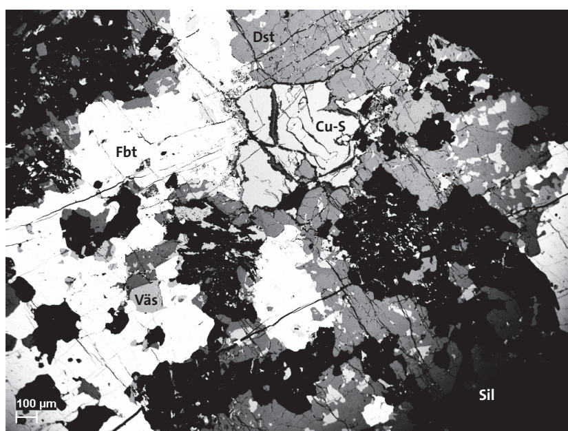
Figure 55. Back-scattered electron (BSE) image of the REE-rich mineralisation from Stålklockan: REE silicates predominate, mainly featuring white fluorbritholite-(Ce) (Fbt), minor medium grey västmanlandite-like mineral (Väs), and similarly medium grey dollaseite-like mineral (Dst), associated with copper sulphides (Cu-S) in skarn silicates (black; Sil), predominantly made up of amphibole. Photo: Erik Jonsson.
