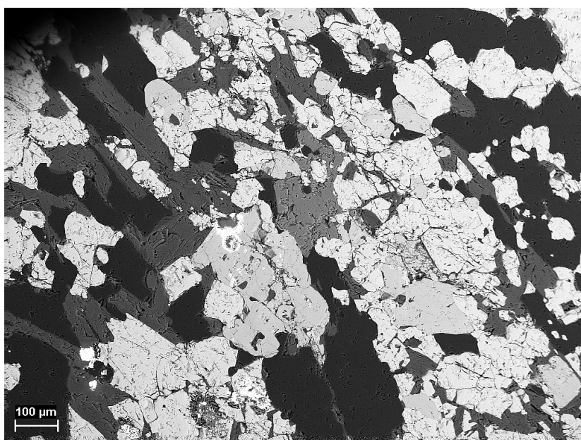
Figure 71. Back-scattered electron (BSE) image showing a silicate-bearing (darkest grey to black) magnetite (lightest grey) ore, with fluorapatite (REE-free; medium grey), locally hosting fine-grained fracture fillings and aggregates of Ca-REE compounds (white, e.g. in an atoll-type texture in the left-central part of the image), and minor allanite-(Ce). The scale bar equals 100 micrometres. Tybble iron mines (6517096/516016). Photo: Erik Jonsson.
