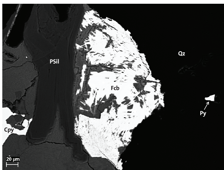
Figure 80. Back-scattered electron (BSE) image showing fracture-hosted, radial aggregates of an REE fluorocarbonate close to synchysite-(Y) (white; Fcb) associated with phyllosilicate minerals and quartz (dark grey to black; PSil and Qz) as well as minor sulphides (lightest grey to white; Cpy = chalcopyrite, Py = pyrite). The scale bar equals 20 micrometres. Bredåsen (6689355/ 661045). Photo: Erik Jonsson.
