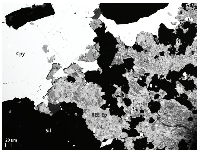
Figure 78. Back-scattered electron (BSE) image showing REE-enriched epidote to allanite-(Ce) (grey-mottled; REE-Ep) with abundant, small BSE-white inclusions which consist of an Y-Fe-silicate (gadolinite-group mineral?) intergrown with skarn silicates and quartz (black; Sil) and in contact with chalcopyrite (white; Cpy). The scale bar equals 20 micrometres. Bredåsen (6689355/ 661045). Photo: Erik Jonsson.
