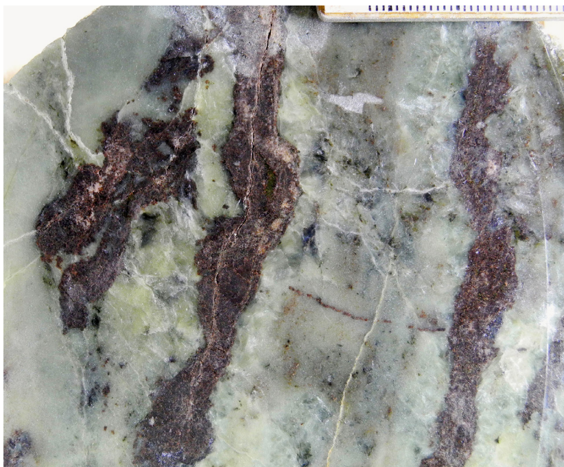
Figure 64. Hand specimen image of a sawn and lightly polished slab showing deformed, partly folded and recrystallised bands of fine-grained REE silicate - fluoro-carbonate mineralisation, dominated by dollaseite-(Ce), in a palest green amphibole-riddled (skarn-altered) dolomitic marble. Heavy black lines in the scale bar in the upper right part of the image are cm markings; fine lines represent millimetres. Johanna mine (6658660/550883), Norberg area. Photo: Per Nysten.
