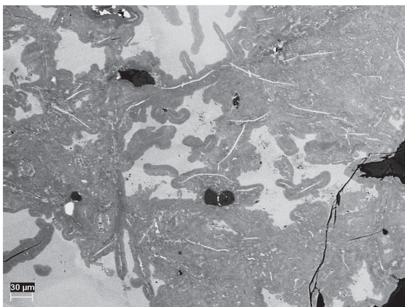
Figure 5. Back-scattered electron (BSE) scanning electron microscope image of a radioactive and hence metamict Y-HREE-U-Ti-Nb oxide from the Flintgruvan (1) pegmatite, Dalarna (6694334/522455), which has experienced extensive, probably fluid-mediated alteration. The light grey to nearly white fields represent remnants of the metamict “original” mineral, which has been largely replaced by a darker phase along gently curving fracture networks. These are in turn partly infilled with a very BSE-light/white phase, a late-formed radiogenic galena. Photo: Erik Jonsson.
