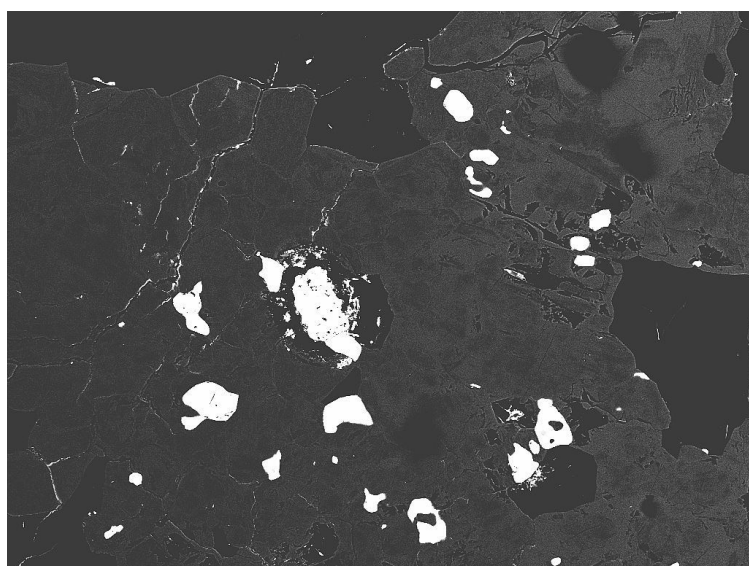
Figure 18. Back-scattered electron (BSE) image of an REE mineralised sample from the Tåresåive mineralisation (7421196/709317). The dark grey to black groundmass predominantly comprises REE epidote/allanite-(Ce), quartz, and mica. The majority of subrounded, white grains are monazite-(Ce), with minor xenotime-(Y) and REE fluorocarbonates. The left central heterogeneous grain/aggregate consists of a core portion of a partially altered U-Pb-Th-U-rich phase, surrounded by two monazite grains. Photo: Erik Jonsson.
