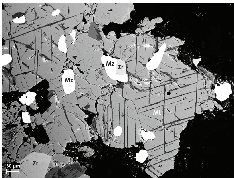
Figure 69. Back-scattered electron (BSE) image of magnetite aggregates (medium grey; Mt) with exsolution lamellae of ilmenite (black, crystallographically oriented) and abundant, subrounded inclusions of monazite-(Ce) (white; Mz) and zircon (light grey; Zr). Silicate minerals are dark grey to black. The scale bar equals 30 micrometres. Sveafallen (6563296/467479). Photo: Erik Jonsson.
