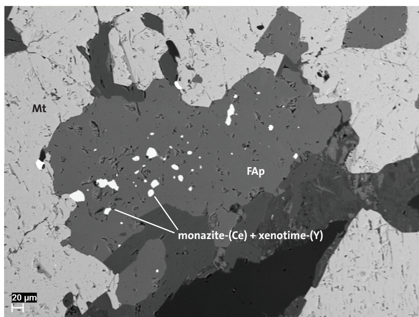
Figure 74. Back-scattered electron (BSE) image showing essentially anhedral fluorapatite (medium grey; FAp) associated with minor silicates (darker grey to black) intergrown in magnetite (lightest grey; Mt). This fluorapatite carries numerous subhedral inclusions of xenotime-(Y) and monazite-(Ce) (both white), texturally very similar to several REE-enriched apatite-iron oxide ores that have been studied. The scale bar equals 20 micrometres. Hylleled iron mines (6433571/580704). Photo: Erik Jonsson.
