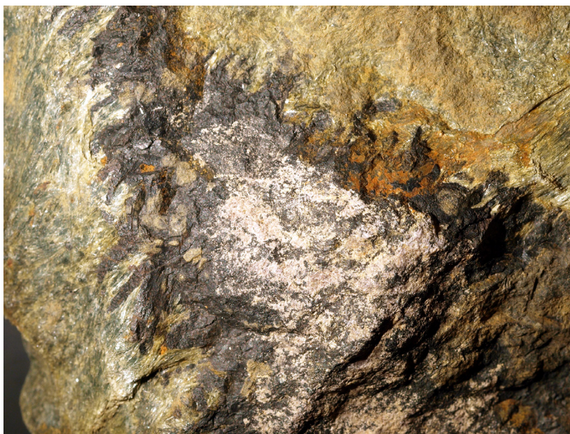
Figure 51. A characteristic REE-rich assemblage from the Nya Bastnäs field: a fine-grained, light-coloured mass of cerite-(Ce), with minor intergrown ferriallanite-(Ce) and bastnäsite-(Ce) is rimmed by coarser-grained ferriallanite-(Ce), within a pale green amphibole-dominated skarn. The cerite-dominated material in the centre has become dull and whitish due to post-mining surface alteration. Photo: Erik Jonsson.
