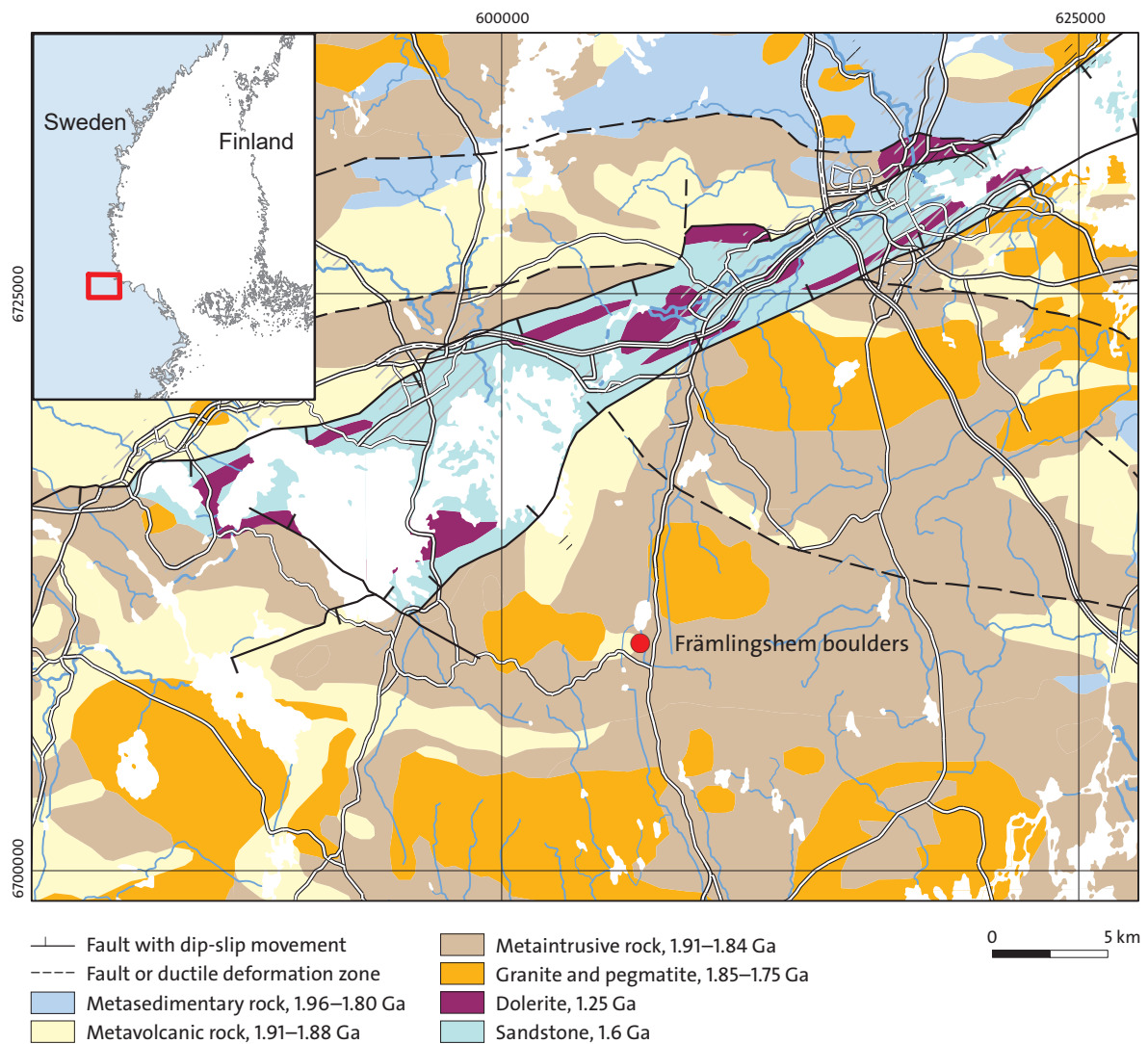
Figure 30. Simplified bedrock geology map showing the location of the Främlingshem boulders (6709872/605974), in relation to the poorly exposed Gävle graben structure.
