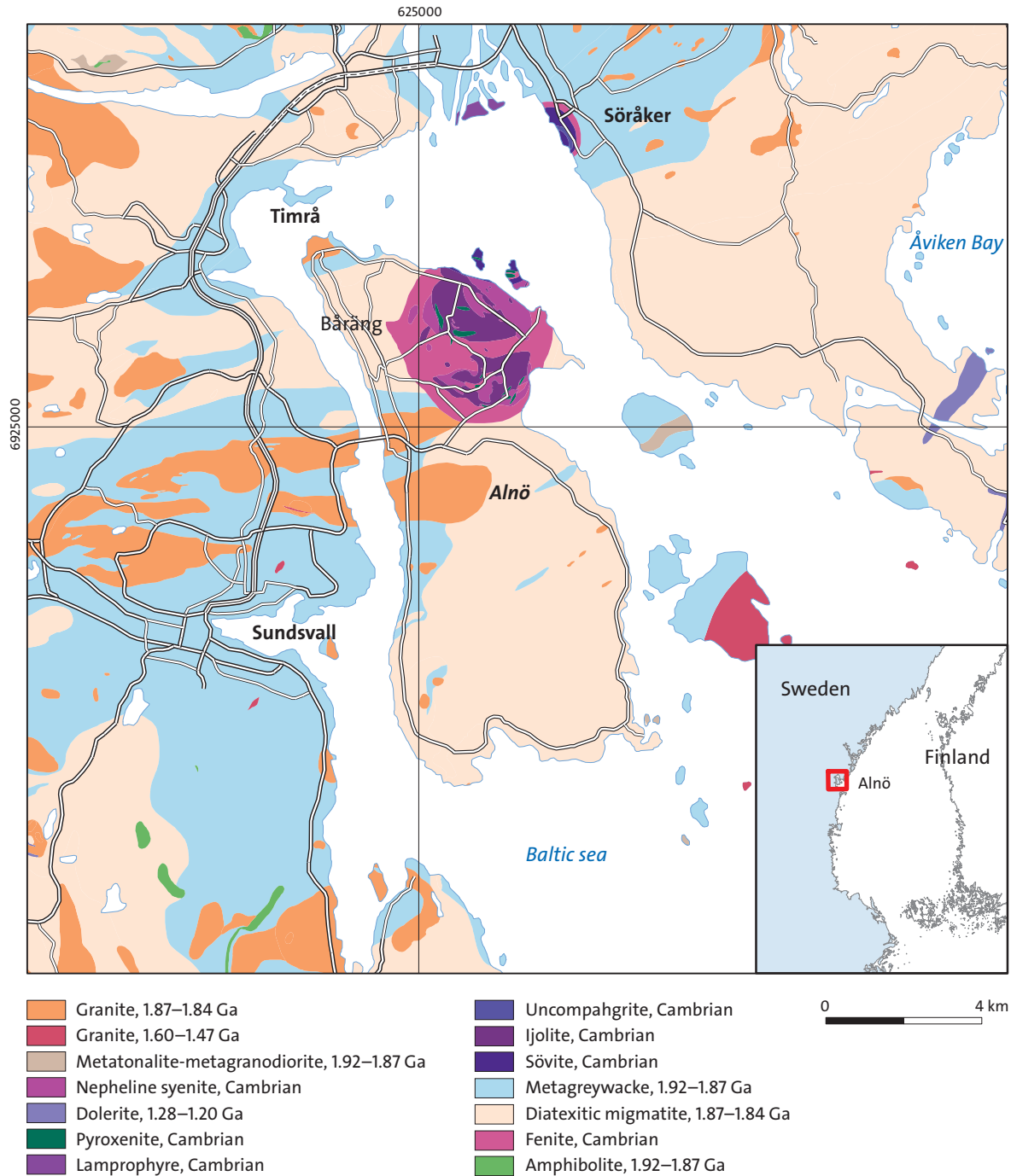
Figure 23. Simplified bedrock geology map of the Alnö complex and surrounding areas.
