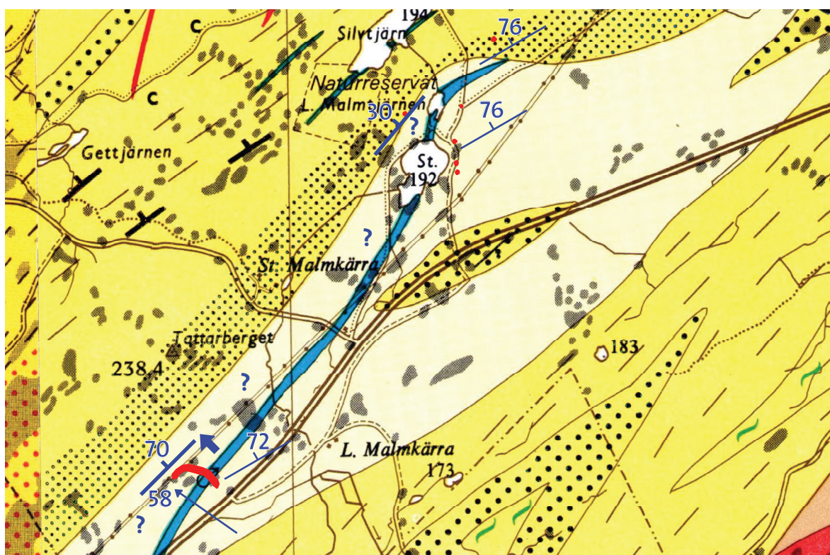
Figure 100. The geology of the Malmjärnen-Plåtängsgruvan area. The background is the bedrock map by Ambros (1988). Red dots and lines (except those in the uppermost part of the map) denote outcrops investigated in this study. The arrow denotes interpreted younging direction. Additional structural measurements in blue. Question marks west of carbonate rock horizon (in blue) denote our interpretation that the rocks here are generally less mica-altered than those east of it. The view is approximately 4.2 km wide. N is up.
