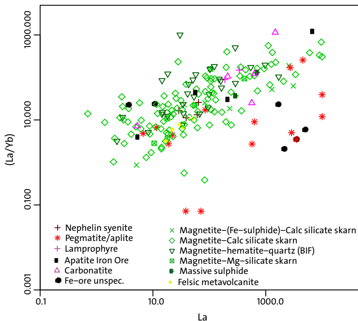
Figure 92. Bivariate plot of La versus La/Yb for the samples analysed.
