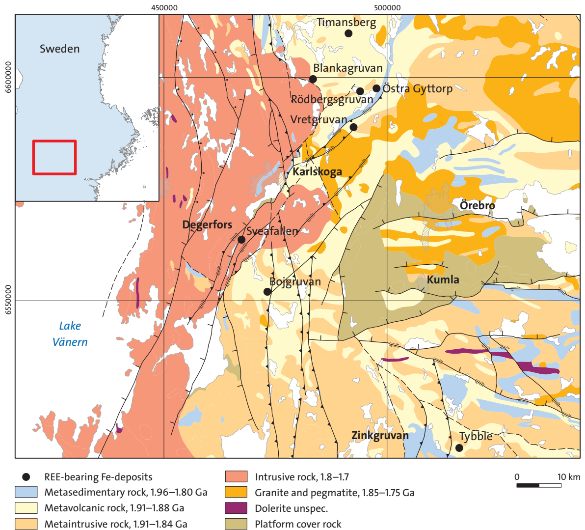
Figure 67. Simplified bedrock geology map showing locations of mines with REE mineralisation in the southwestern to southernmost part of the Bergslagen ore province, including the southwesternmost part of the REE line, and the Zinkgruvan mine for reference.
