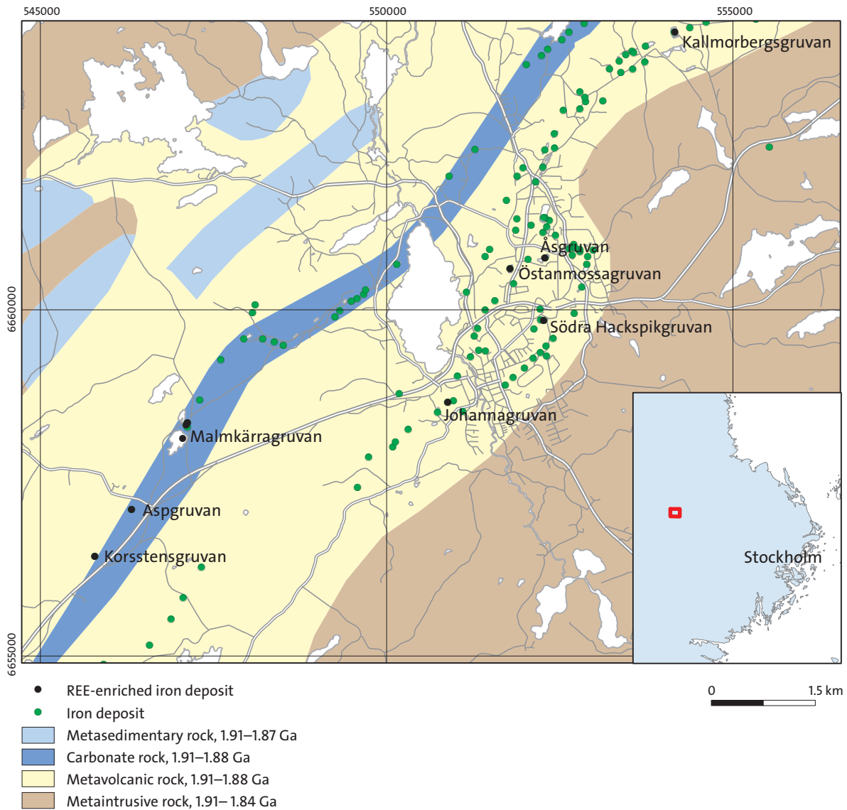
Figure 63. Simplified bedrock geology map showing locations of mines in the Norberg area, northeastern part of the REE line, highlighting those with known REE mineralisation.
