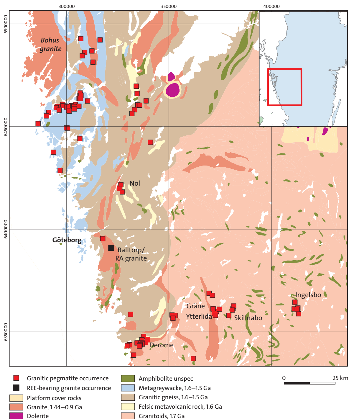
Figure 7. Simplified bedrock geology map showing locations of granitic pegmatites (quarries) and granitoids in southwestern Sweden; REE-enriched occurrences mentioned in the text are named.
