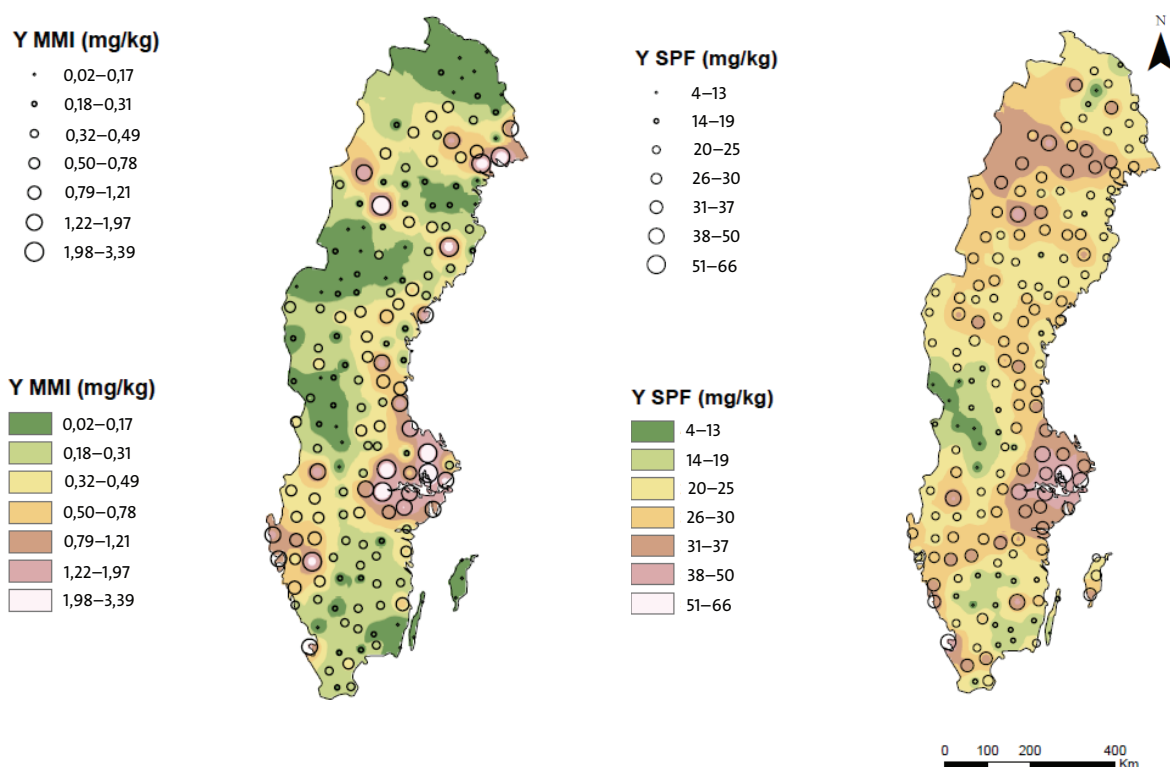
Figure 89. Colour map for Y in Ap soil in Sweden for MMI® extraction and sodium peroxide fusion technique (SPF)
