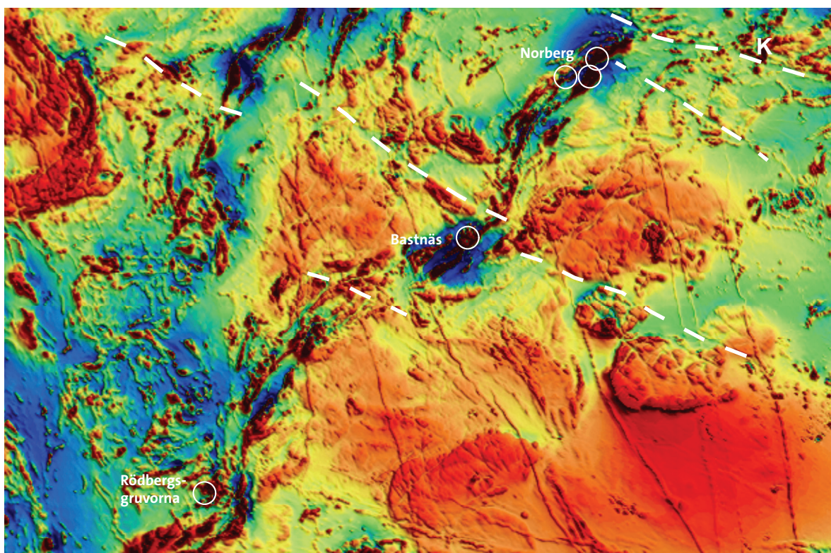
Figure 102. Aeromagnetic anomaly map of the REE line area. White circles mark locations of known REE mineralisations. Broken white lines mark interpreted lineaments. K marks the location of the Knutsbo REE deposit.
