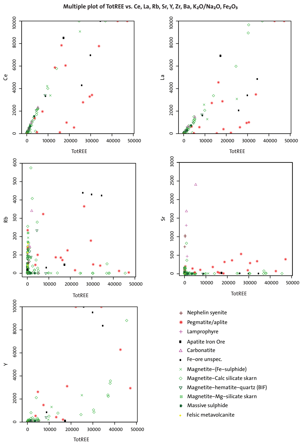
Figure 94. Plots of some elements versus total REE in the samples analysed. The figure continues on the next page.
