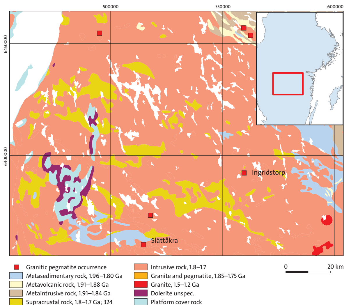
Figure 8. Simplified bedrock geology map showing locations of quarried granitic pegmatites in part of southeastern Sweden; REE-enriched occurrences mentioned in the text are named.
