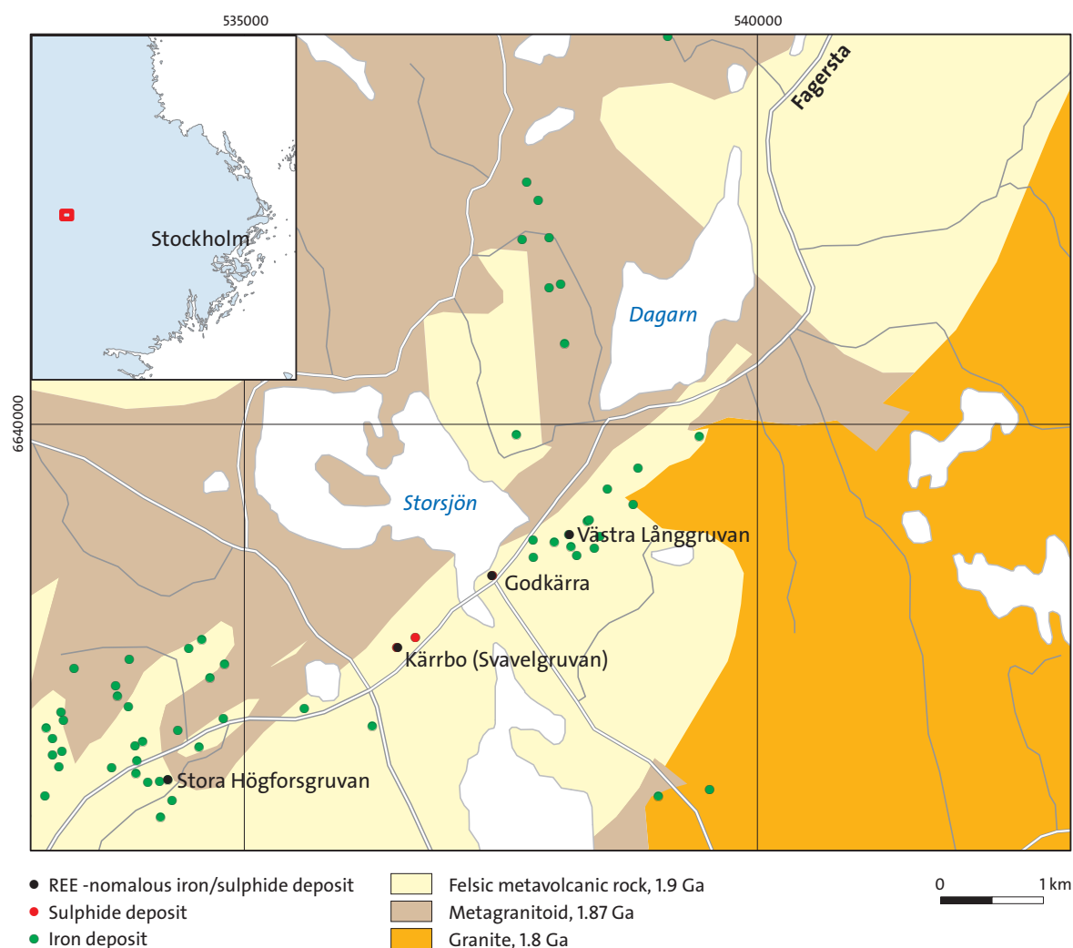
Figure 58. Simplified bedrock geology map showing the locations of mines in the area northeast of Bastnäs, Riddarhyttan area, in the central part of the REE line, highlighting those with REE enrichment.
