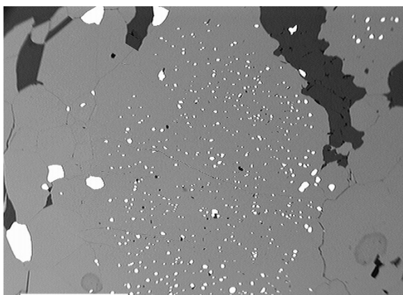
Figure 39. Back-scattered electron (BSE) image of fluorapatite (grey) in magnetite-apatite ore from the Export field, Grängesberg. The small white inclusions in the centre of the image consist of monazite-(Ce) and minor xenotime-(Y). Larger grains or crystals in the outer parts of the fluorapatite are monazite-(Ce). This texture is interpreted to be the result of fluid-mediated remobilisation of the originally fluorapatite-hosted REEs into later-formed REE phosphates, subsequently in part modified by Ostwald ripening-type processes, which led to the growth of fewer and bigger monazites in the outer part of the fluorapatite grains. The white scale bar at lower left equals 200 micrometres. Photo: Erik Jonsson.
