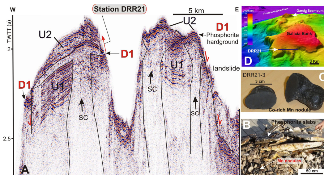
Figure 4. W-E A05 multichannel seismic profile across mounds and canyons along southern Galicia Bank. Vertical exaggeration is X18 ( V = 2.0 km/s). Mounds with an internal chaotic and indistinct seismic reflection pattern and development of “seismic chimneys (SC)” that crosscut the D1 discontinuity and affect U1 and partially U2 units. (b) Suite of phosphorite slabs and Co-rich Mn nodules dredged at station DRR21. (c) Cut sections of Co-rich Mn nodules. (d) Location of seismic profile and dredge station.
