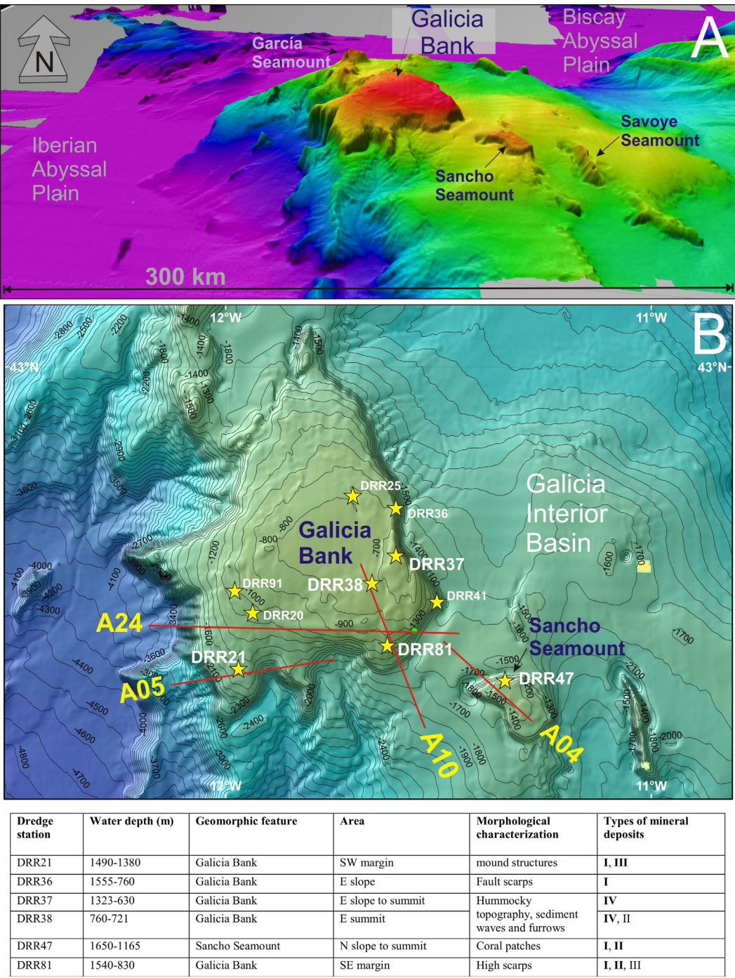
Figure 2. (top) Three-dimensional multibeam bathymetric image (Simrad EM12-120S), Fledermaus visualization of the seabed structure map in the study area. Viewing direction is from the South. (bottom) Data sets used, including dredge hauls (stars), multichannel seismic reflection lines (red lines), and simplified bathymetry. Table below: data set of the most relevant morphological characteristics of the dredge stations selected for this study.
