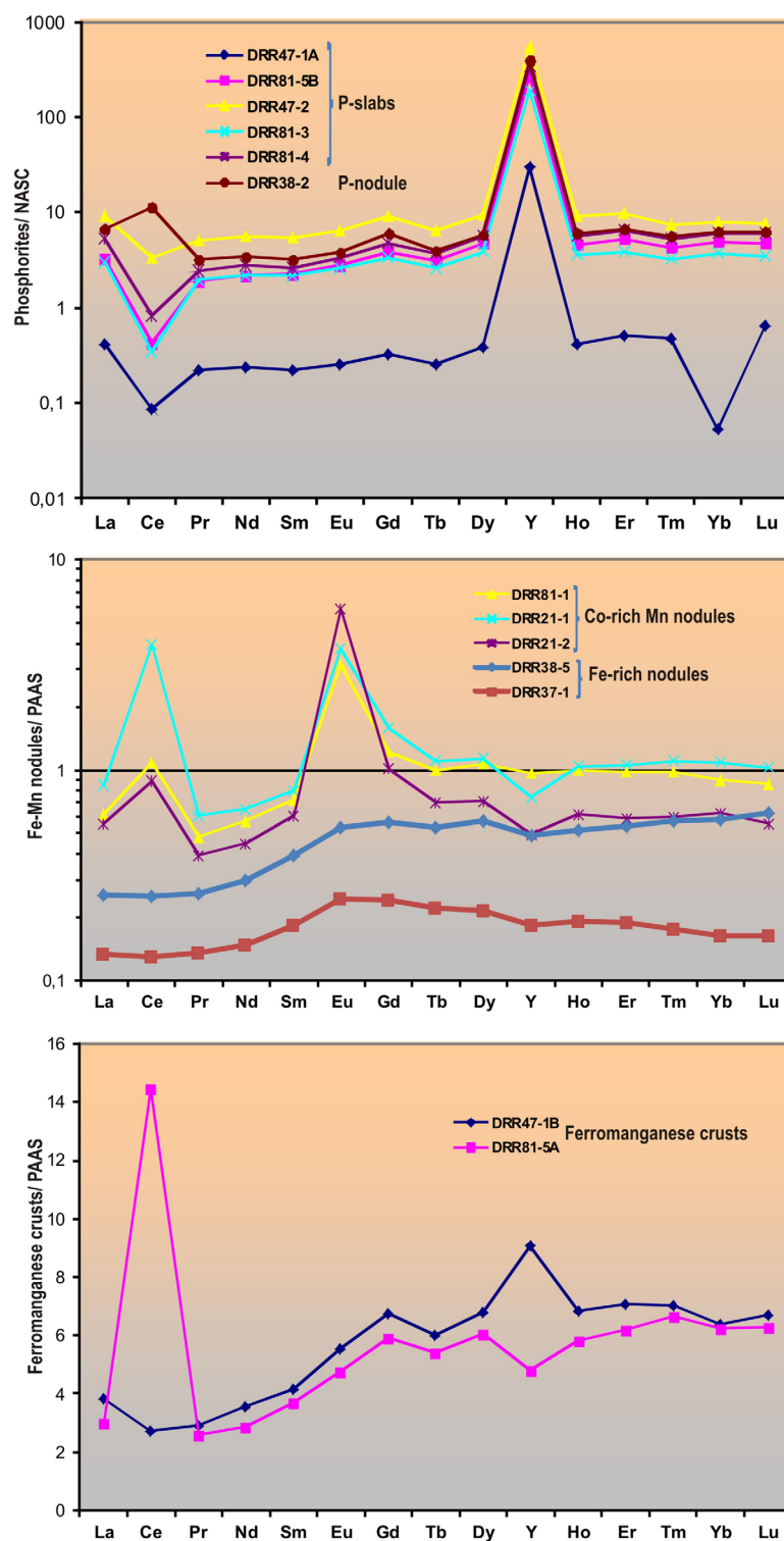
Figure 8. PAAS-normalized and NASC-normalized REY element plots for phosphorites, Co-rich Mn nodules, Fe-rich nodules, and Fe-Mn crusts.
