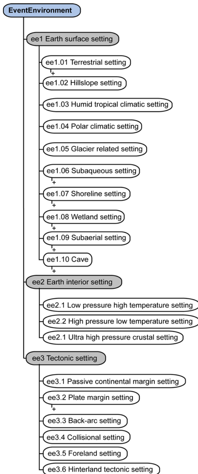
Figure 4-7: Hierarchical overview representation of the 1G-E vocabulary for EventEnvironment.
